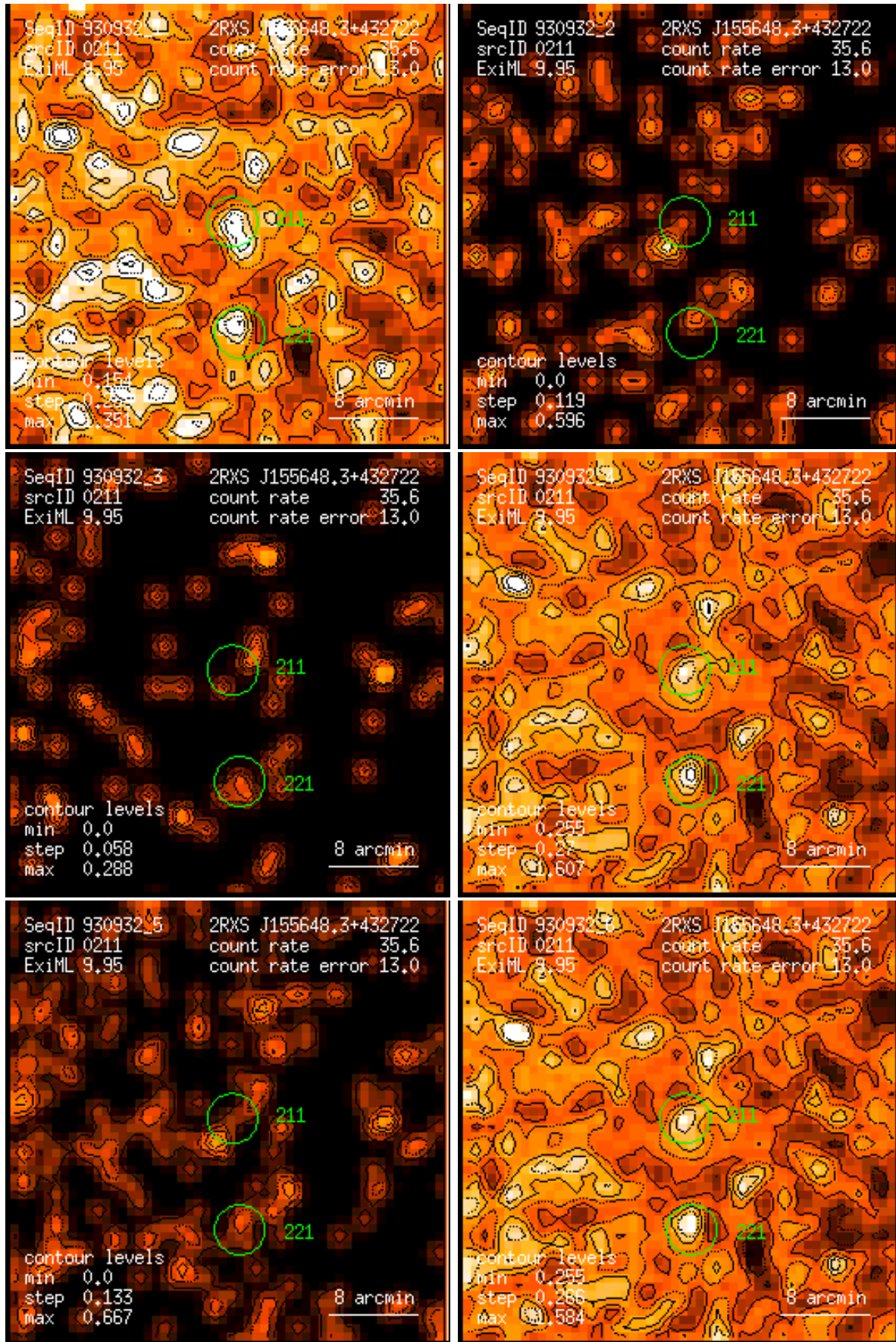
Figure 211: RASS 930932: detection 0211: band rate images, Gaussian filter: (1) PSPC channels 11 – 41, (2) 52 – 90, (3) 91 – 201, (4) 11 – 235, (5) 52 – 201, (6) 11 – 201. Broad band rates in counts/ks. Band rate contour levels in counts/ks/arcmin 2 .
