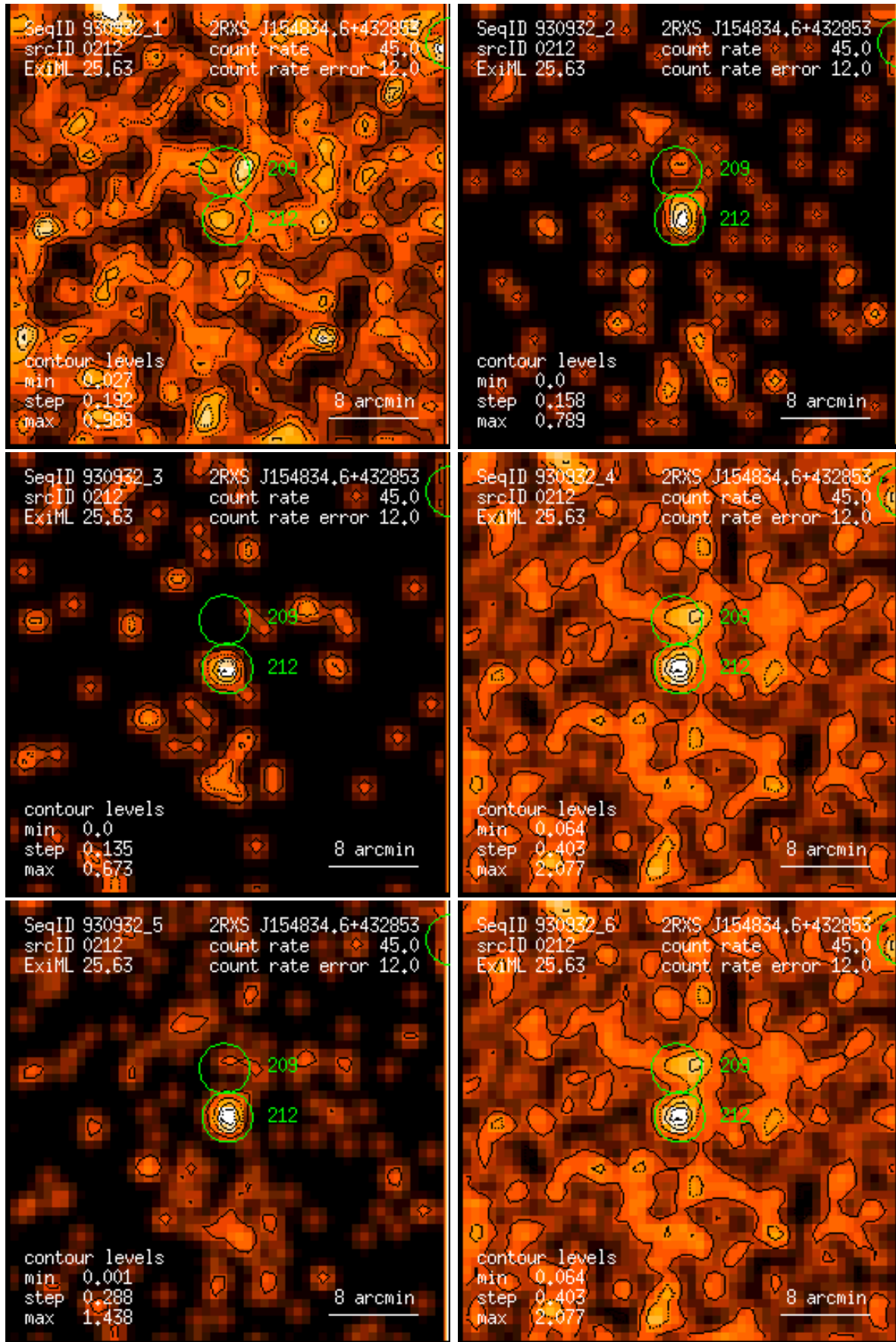
Figure 212: RASS 930932: detection 0212: band rate images, Gaussian filter: (1) PSPC channels 11 – 41, (2) 52 – 90, (3) 91 – 201, (4) 11 – 235, (5) 52 – 201, (6) 11 – 201. Broad band rates in counts/ks. Band rate contour levels in counts/ks/arcmin 2 .
