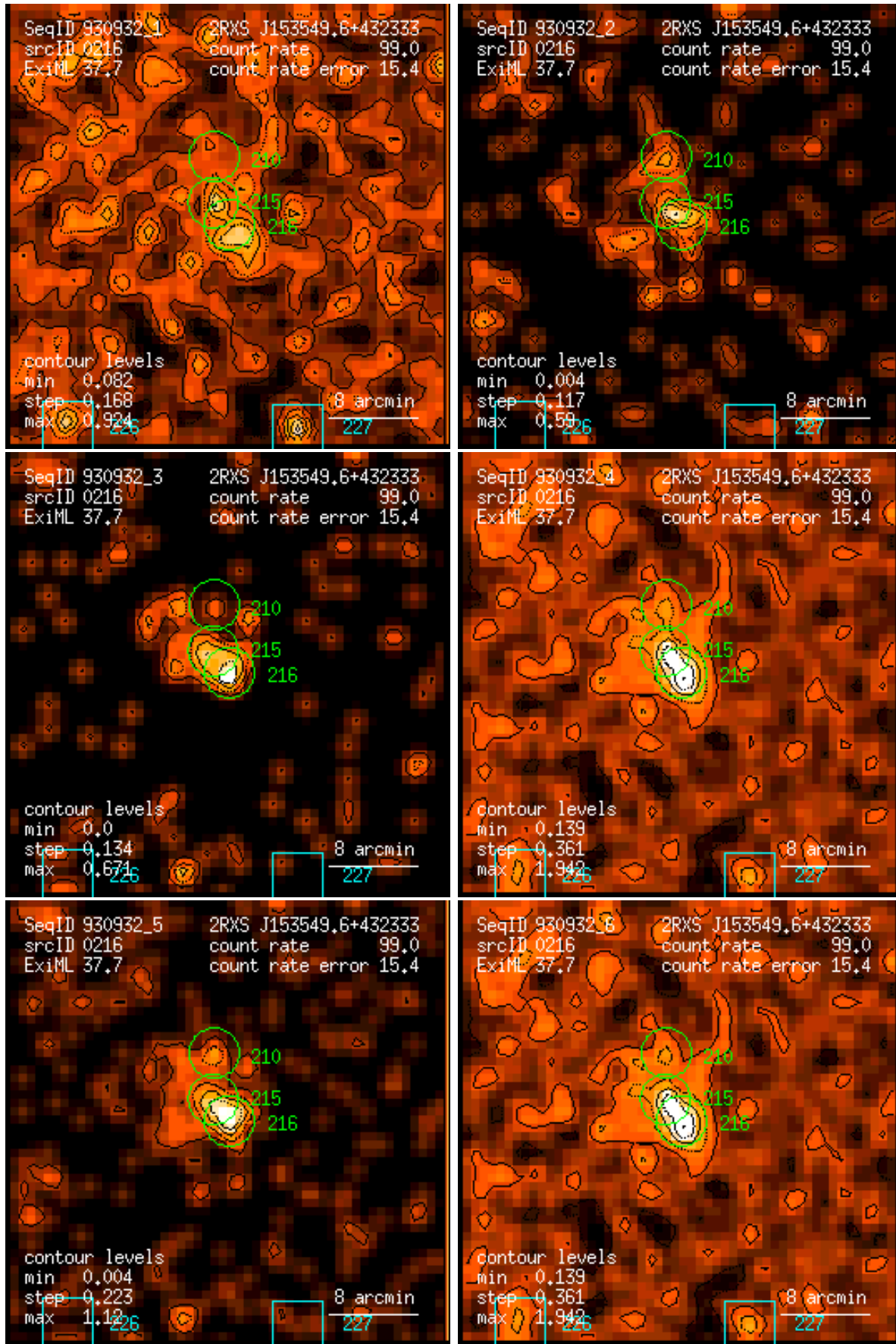
Figure 216: RASS 930932: detection 0216: band rate images, Gaussian filter: (1) PSPC channels 11 – 41, (2) 52 – 90, (3) 91 – 201, (4) 11 – 235, (5) 52 – 201, (6) 11 – 201. Broad band rates in counts/ks. Band rate contour levels in counts/ks/arcmin 2 .
