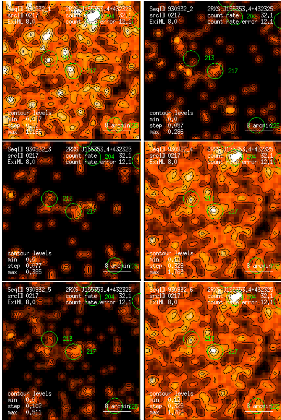
Figure 217: RASS 930932: detection 0217: band rate images, Gaussian filter: (1) PSPC channels 11 – 41, (2) 52 – 90, (3) 91 – 201, (4) 11 – 235, (5) 52 – 201, (6) 11 – 201. Broad band rates in counts/ks. Band rate contour levels in counts/ks/arcmin 2 .
