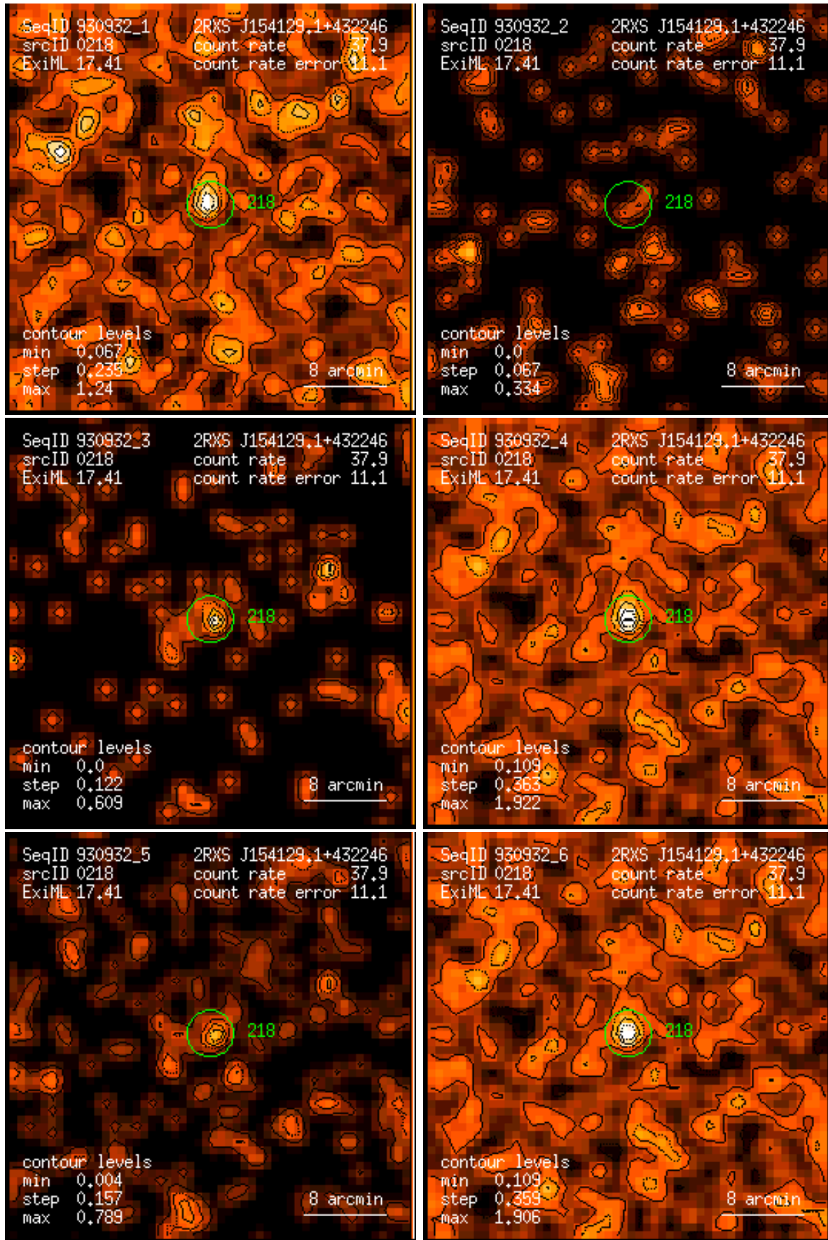
Figure 218: RASS 930932: detection 0218: band rate images, Gaussian filter: (1) PSPC channels 11 – 41, (2) 52 – 90, (3) 91 – 201, (4) 11 – 235, (5) 52 – 201, (6) 11 – 201. Broad band rates in counts/ks. Band rate contour levels in counts/ks/arcmin 2 .
