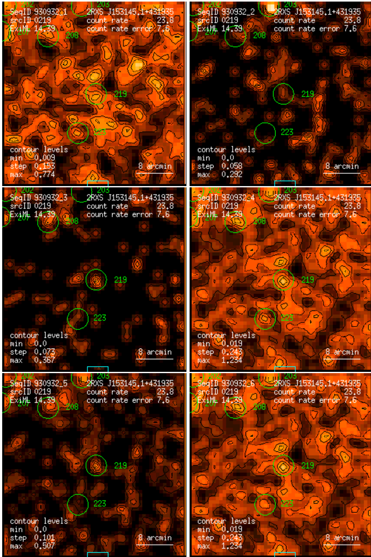
Figure 219: RASS 930932: detection 0219: band rate images, Gaussian filter: (1) PSPC channels 11 – 41, (2) 52 – 90, (3) 91 – 201, (4) 11 – 235, (5) 52 – 201, (6) 11 – 201. Broad band rates in counts/ks. Band rate contour levels in counts/ks/arcmin 2 .
