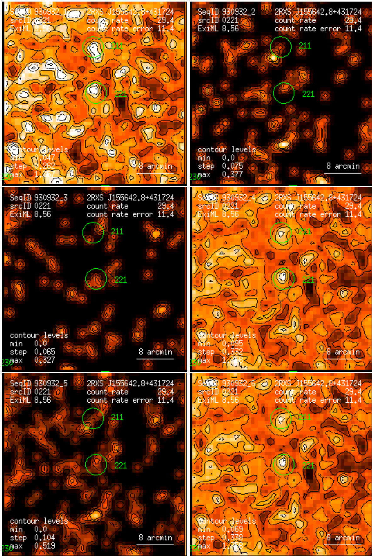
Figure 221: RASS 930932: detection 0221: band rate images, Gaussian filter: (1) PSPC channels 11 – 41, (2) 52 – 90, (3) 91 – 201, (4) 11 – 235, (5) 52 – 201, (6) 11 – 201. Broad band rates in counts/ks. Band rate contour levels in counts/ks/arcmin 2 .
