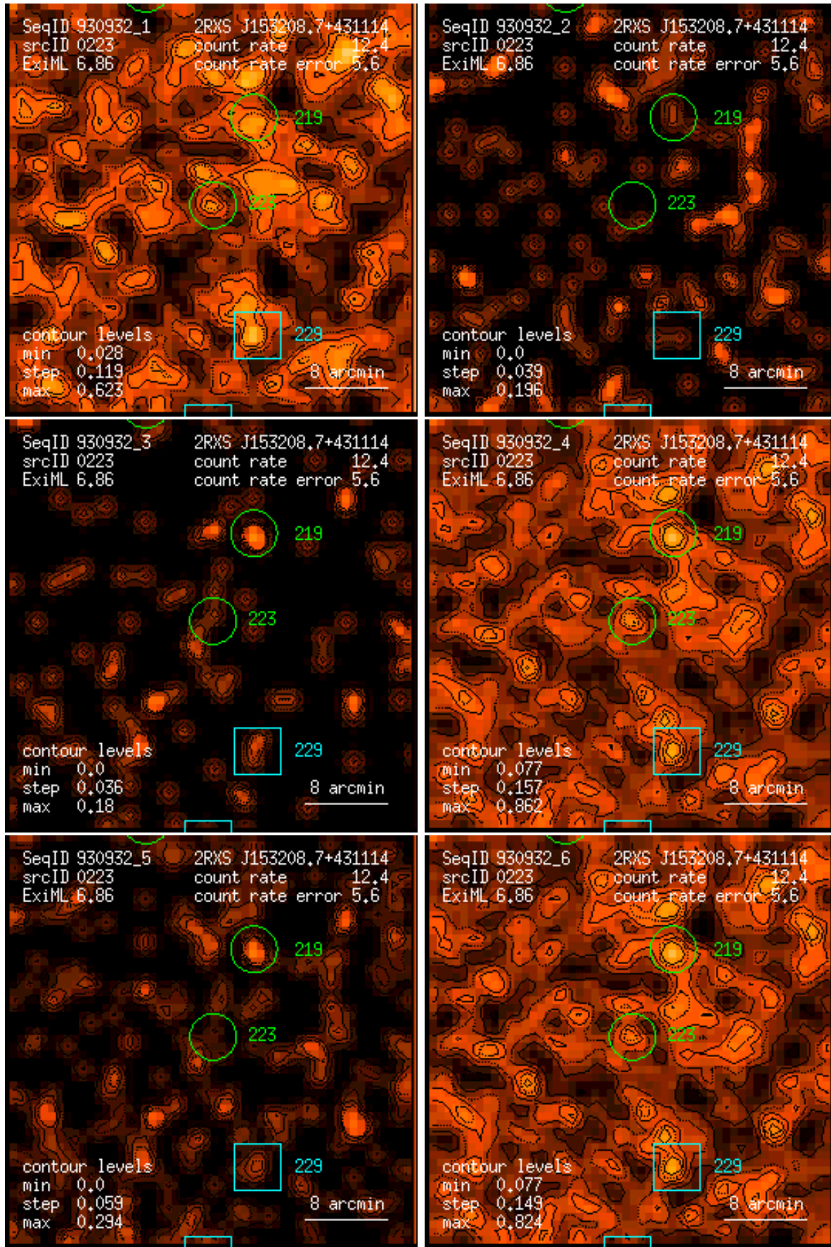
Figure 223: RASS 930932: detection 0223: band rate images, Gaussian filter: (1) PSPC channels 11 – 41, (2) 52 – 90, (3) 91 – 201, (4) 11 – 235, (5) 52 – 201, (6) 11 – 201. Broad band rates in counts/ks. Band rate contour levels in counts/ks/arcmin 2 .
