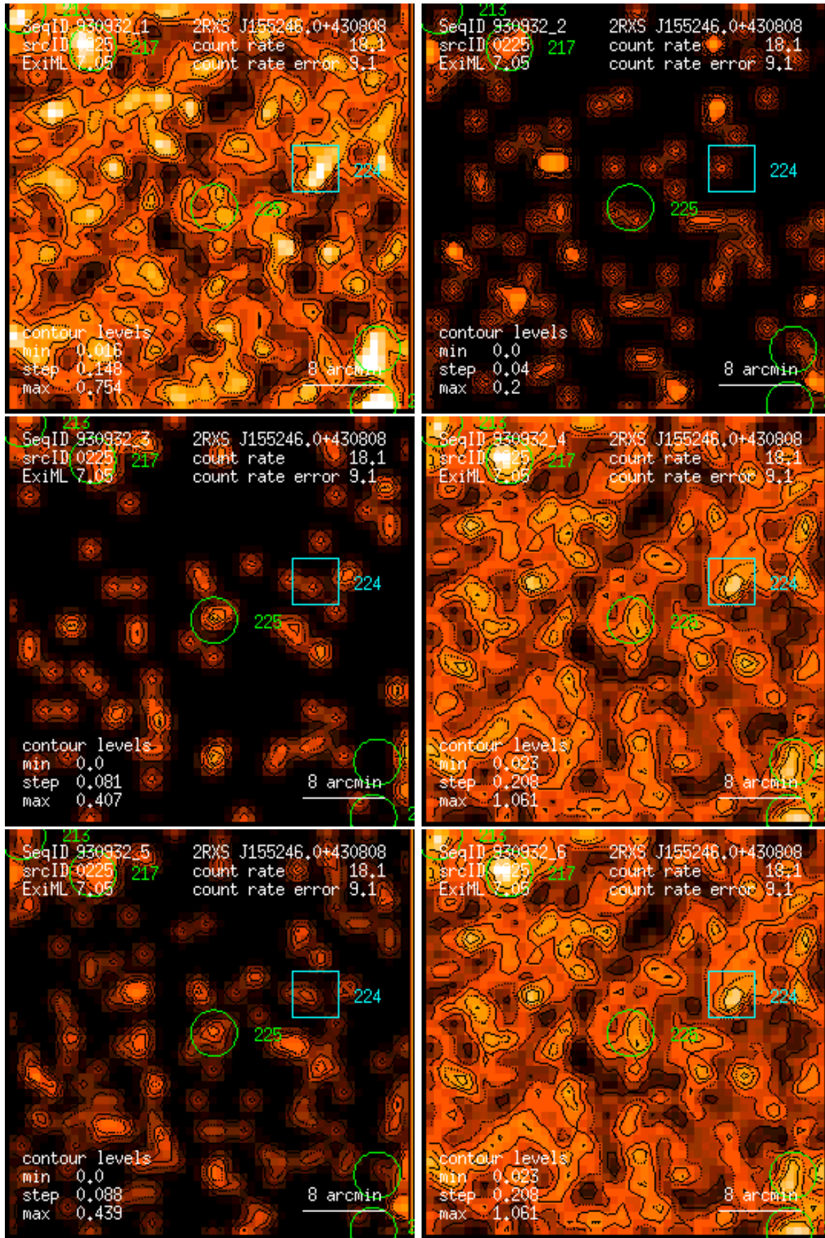
Figure 225: RASS 930932: detection 0225: band rate images, Gaussian filter: (1) PSPC channels 11 – 41, (2) 52 – 90, (3) 91 – 201, (4) 11 – 235, (5) 52 – 201, (6) 11 – 201. Broad band rates in counts/ks. Band rate contour levels in counts/ks/arcmin 2 .
