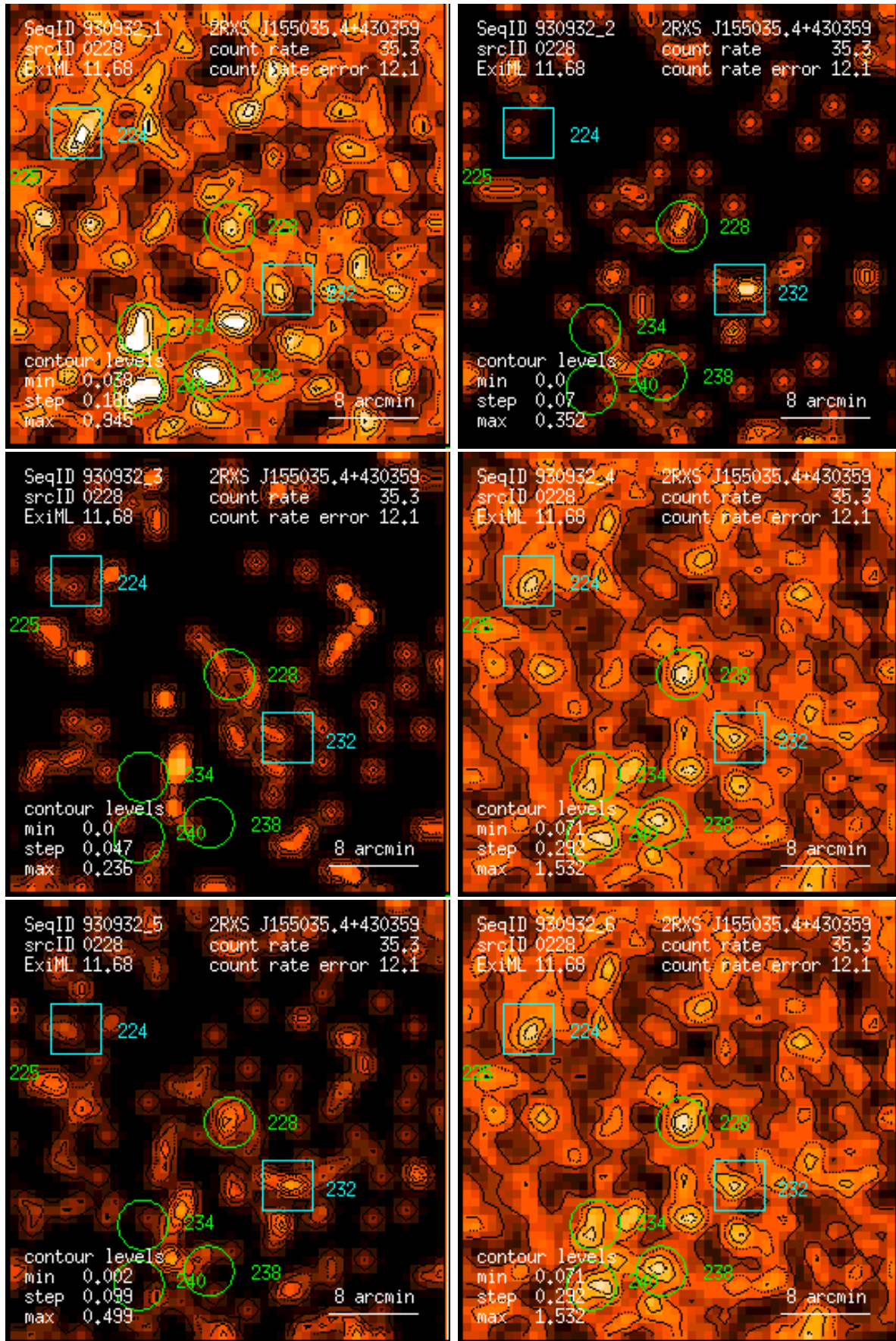
Figure 228: RASS 930932: detection 0228: band rate images, Gaussian filter: (1) PSPC channels 11 – 41, (2) 52 – 90, (3) 91 – 201, (4) 11 – 235, (5) 52 – 201, (6) 11 – 201. Broad band rates in counts/ks. Band rate contour levels in counts/ks/arcmin 2 .
