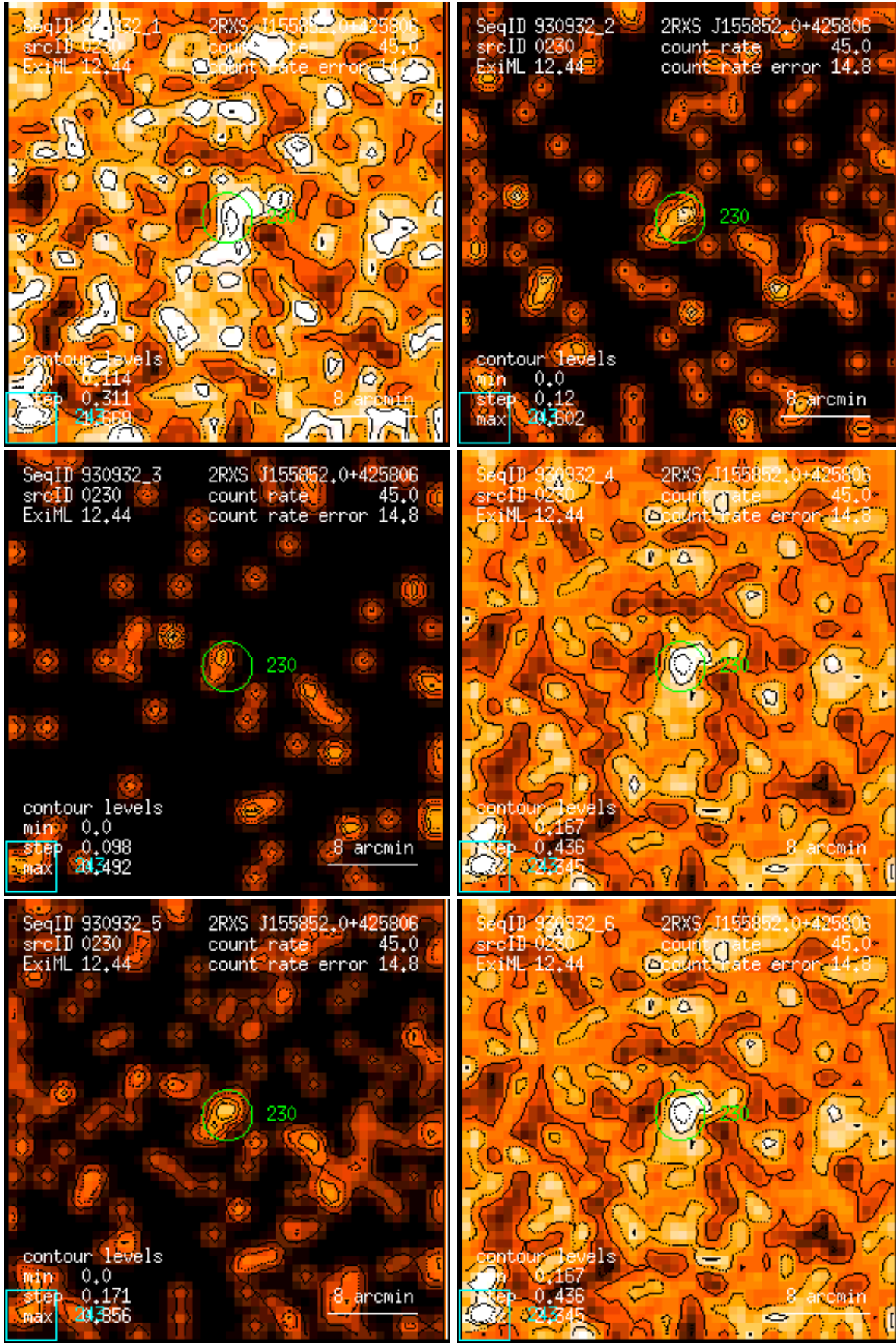
Figure 230: RASS 930932: detection 0230: band rate images, Gaussian filter: (1) PSPC channels 11 – 41, (2) 52 – 90, (3) 91 – 201, (4) 11 – 235, (5) 52 – 201, (6) 11 – 201. Broad band rates in counts/ks. Band rate contour levels in counts/ks/arcmin 2 .
