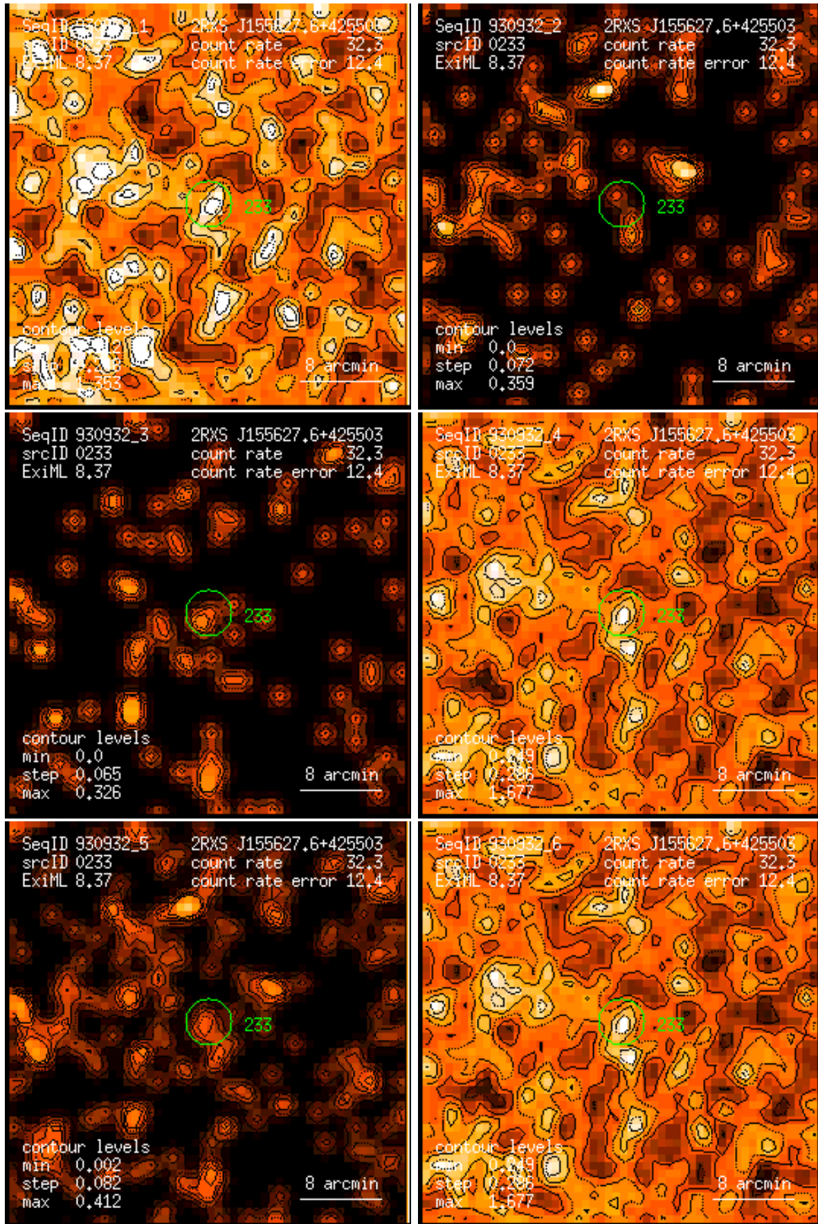
Figure 233: RASS 930932: detection 0233: band rate images, Gaussian filter: (1) PSPC channels 11 – 41, (2) 52 – 90, (3) 91 – 201, (4) 11 – 235, (5) 52 – 201, (6) 11 – 201. Broad band rates in counts/ks. Band rate contour levels in counts/ks/arcmin 2 .
