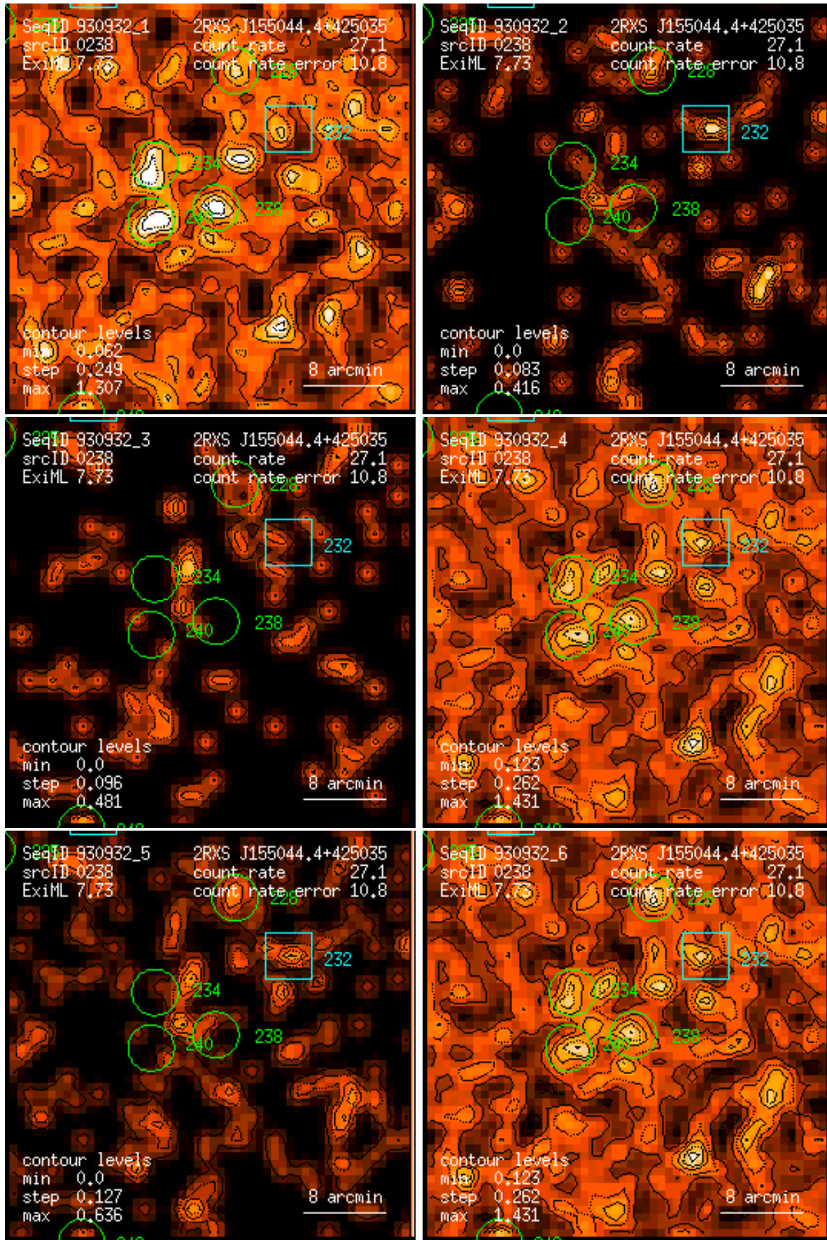
Figure 238: RASS 930932: detection 0238: band rate images, Gaussian filter: (1) PSPC channels 11 – 41, (2) 52 – 90, (3) 91 – 201, (4) 11 – 235, (5) 52 – 201, (6) 11 – 201. Broad band rates in counts/ks. Band rate contour levels in counts/ks/arcmin 2 .
