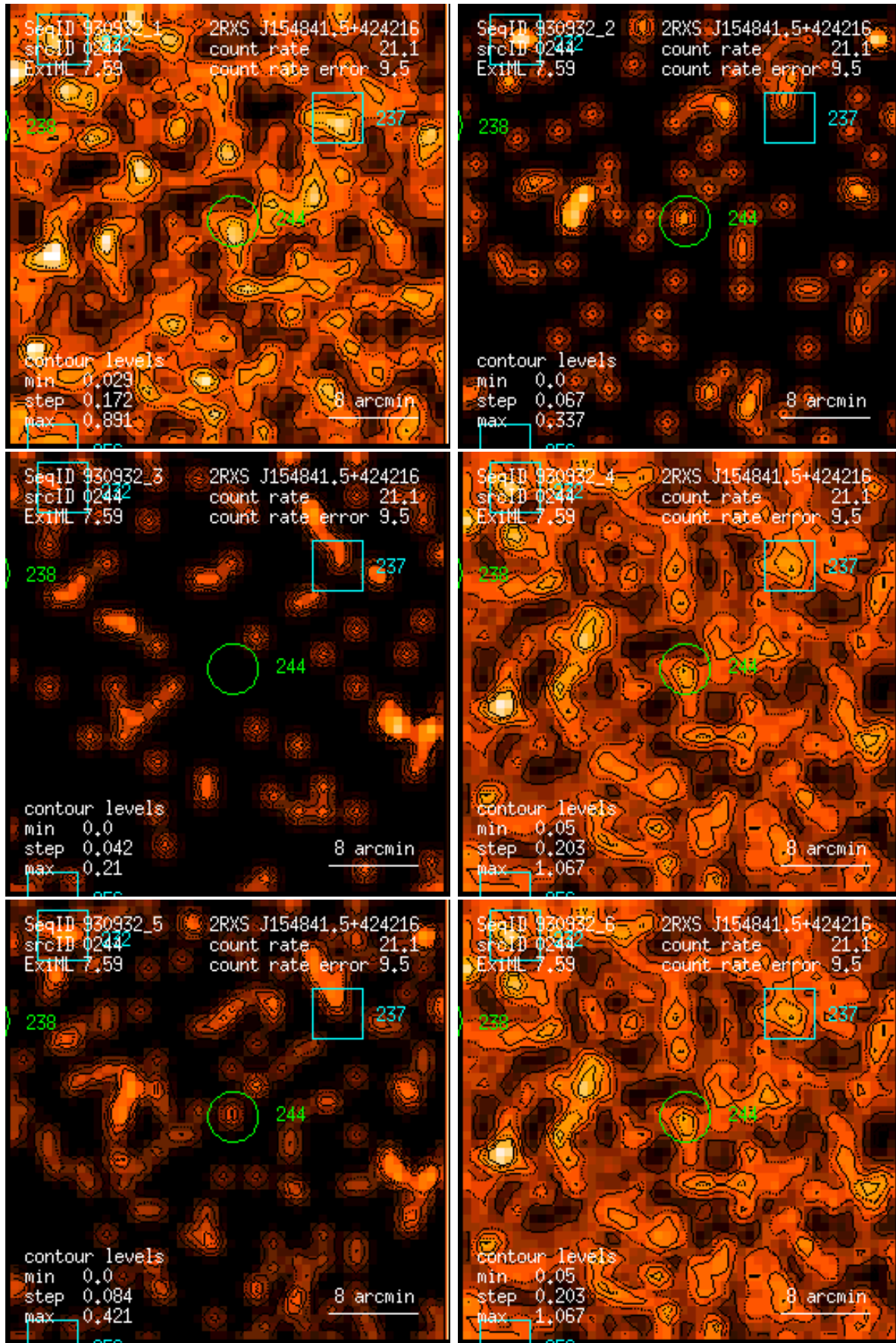
Figure 244: RASS 930932: detection 0244: band rate images, Gaussian filter: (1) PSPC channels 11 – 41, (2) 52 – 90, (3) 91 – 201, (4) 11 – 235, (5) 52 – 201, (6) 11 – 201. Broad band rates in counts/ks. Band rate contour levels in counts/ks/arcmin 2 .
