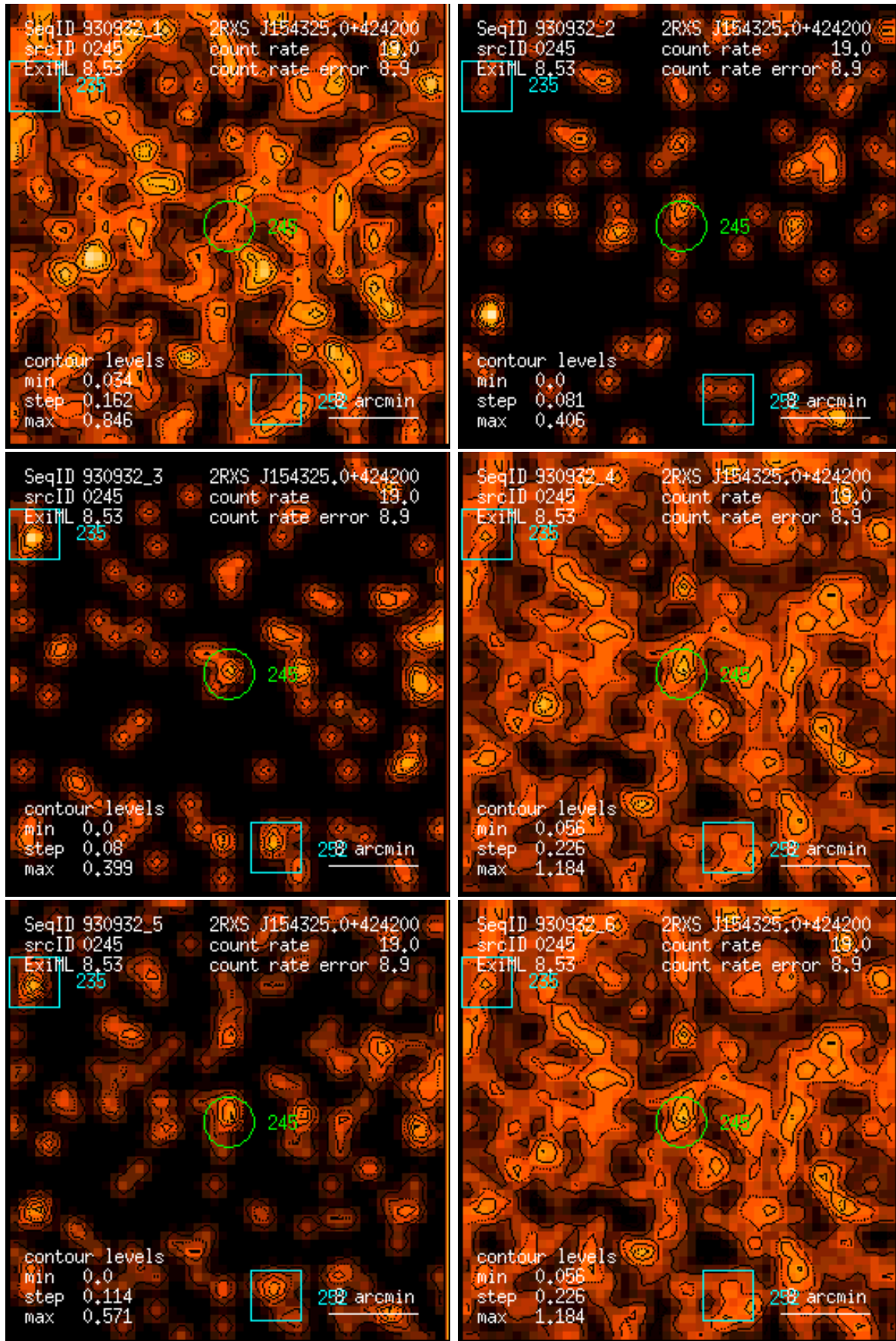
Figure 245: RASS 930932: detection 0245: band rate images, Gaussian filter: (1) PSPC channels 11 – 41, (2) 52 – 90, (3) 91 – 201, (4) 11 – 235, (5) 52 – 201, (6) 11 – 201. Broad band rates in counts/ks. Band rate contour levels in counts/ks/arcmin 2 .
