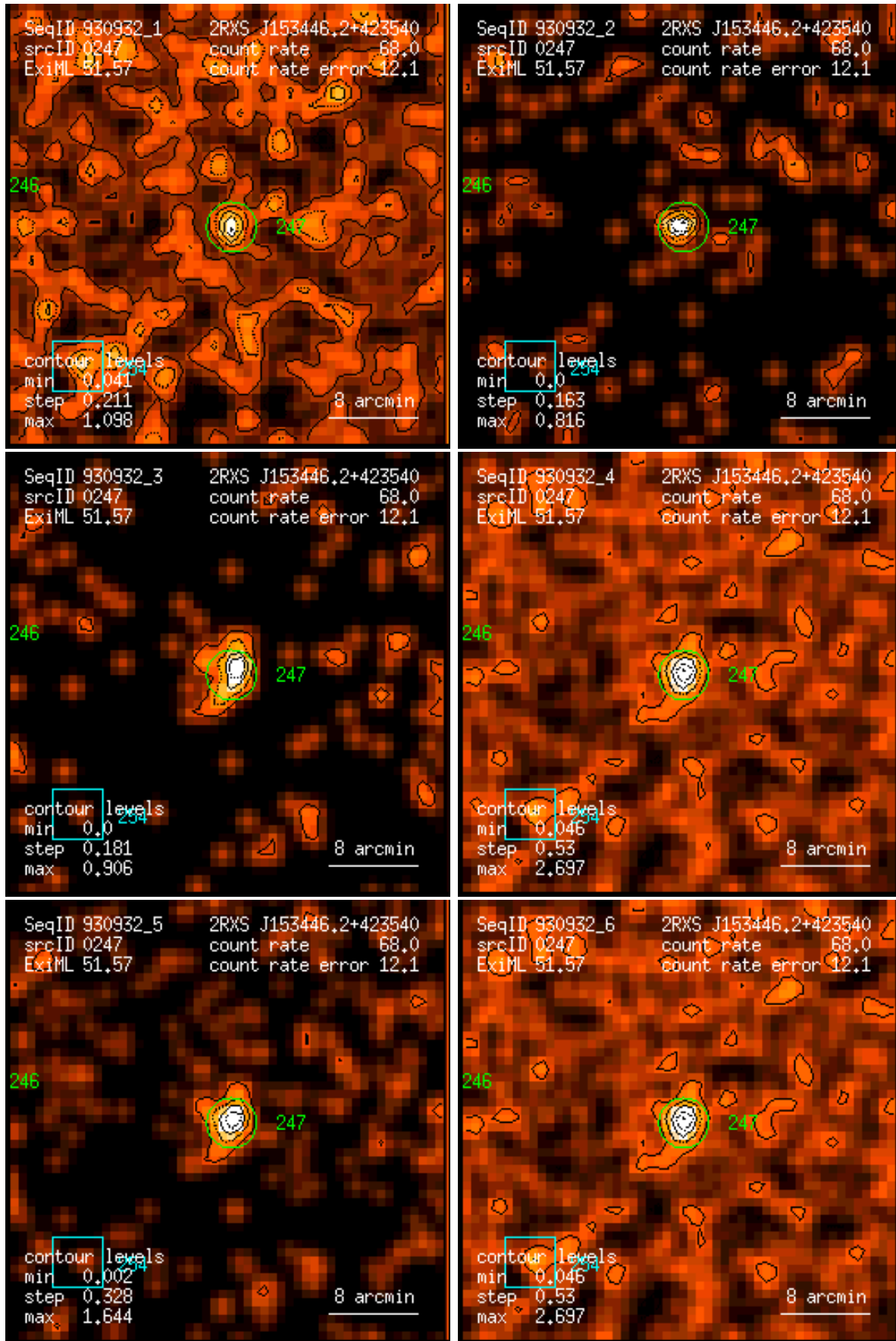
Figure 247: RASS 930932: detection 0247: band rate images, Gaussian filter: (1) PSPC channels 11 – 41, (2) 52 – 90, (3) 91 – 201, (4) 11 – 235, (5) 52 – 201, (6) 11 – 201. Broad band rates in counts/ks. Band rate contour levels in counts/ks/arcmin 2 .
