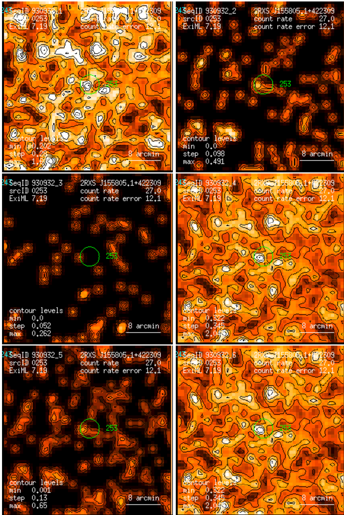
Figure 253: RASS 930932: detection 0253: band rate images, Gaussian filter: (1) PSPC channels 11 – 41, (2) 52 – 90, (3) 91 – 201, (4) 11 – 235, (5) 52 – 201, (6) 11 – 201. Broad band rates in counts/ks. Band rate contour levels in counts/ks/arcmin 2 .
