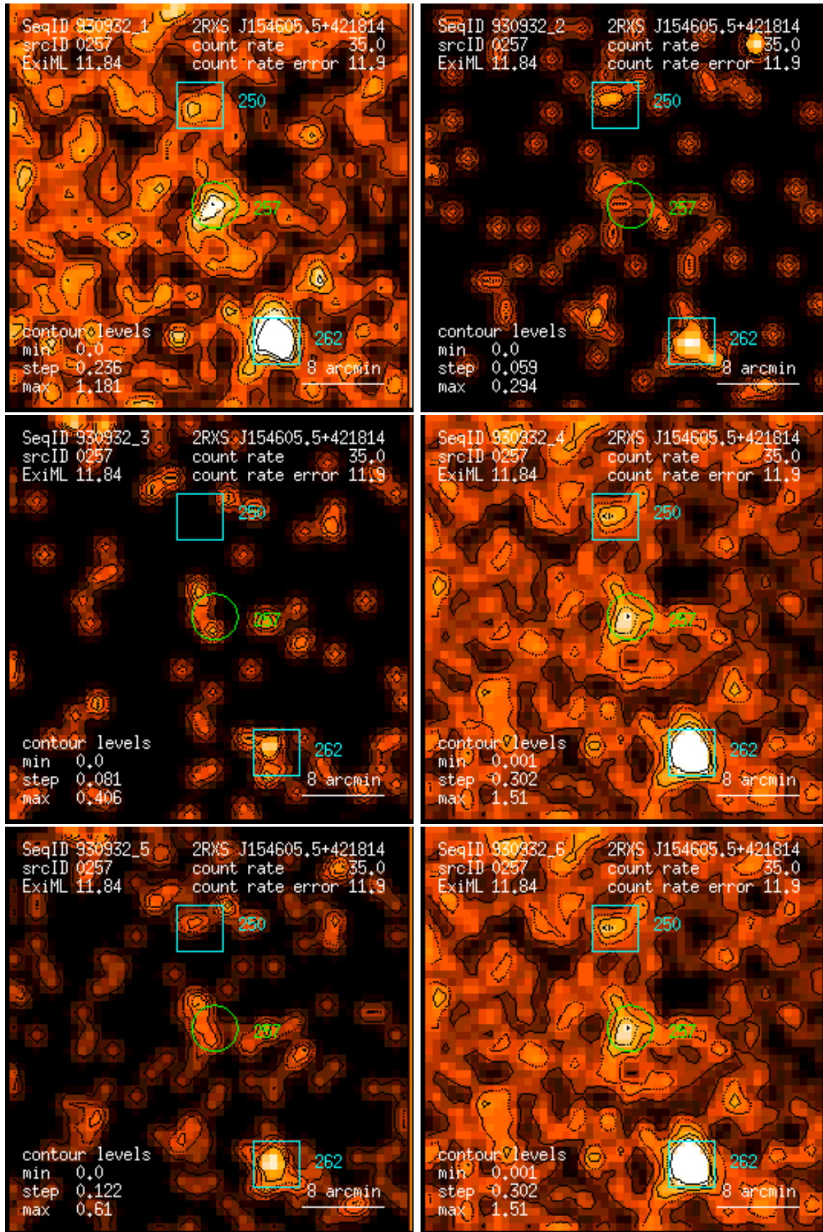
Figure 257: RASS 930932: detection 0257: band rate images, Gaussian filter: (1) PSPC channels 11 – 41, (2) 52 – 90, (3) 91 – 201, (4) 11 – 235, (5) 52 – 201, (6) 11 – 201. Broad band rates in counts/ks. Band rate contour levels in counts/ks/arcmin 2 .
