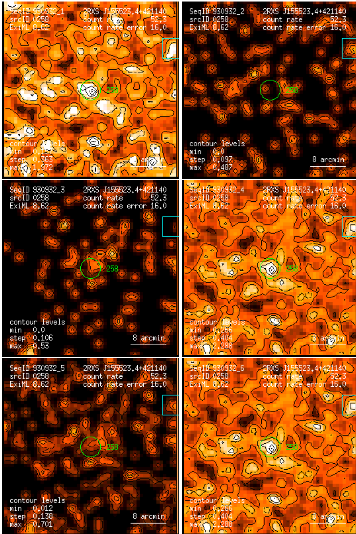
Figure 258: RASS 930932: detection 0258: band rate images, Gaussian filter: (1) PSPC channels 11 – 41, (2) 52 – 90, (3) 91 – 201, (4) 11 – 235, (5) 52 – 201, (6) 11 – 201. Broad band rates in counts/ks. Band rate contour levels in counts/ks/arcmin 2 .
