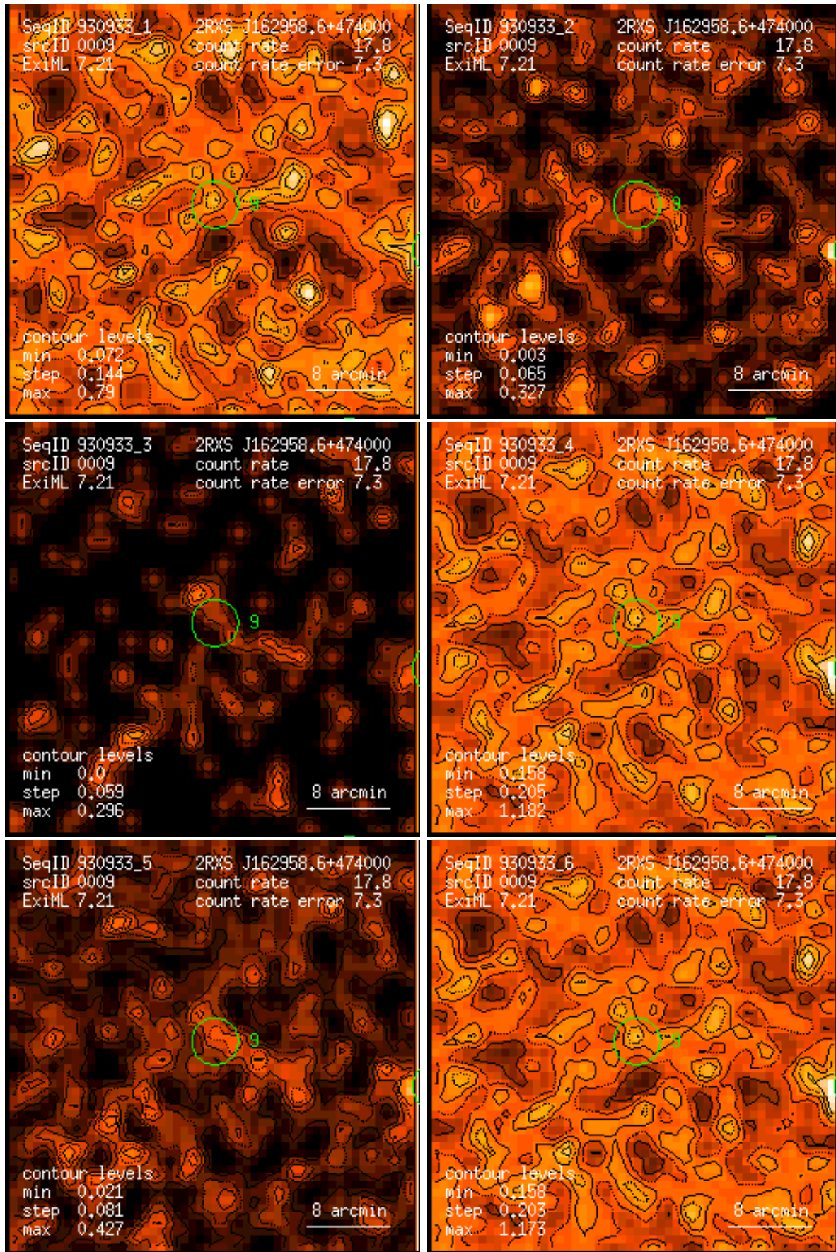
Figure 9: RASS 930933: detection 0009: band rate images, Gaussian filter: (1) PSPC channels 11 – 41, (2) 52 – 90, (3) 91 – 201, (4) 11 – 235, (5) 52 – 201, (6) 11 – 201. Broad band rates in counts/ks. Band rate contour levels in counts/ks/arcmin 2 .
