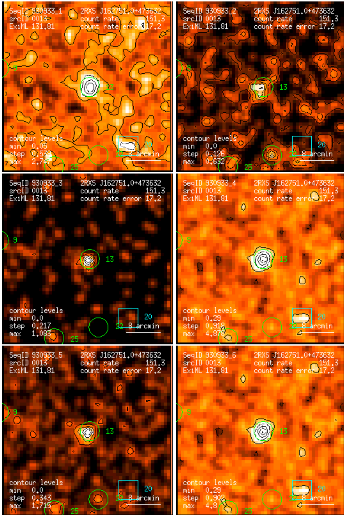
Figure 13: RASS 930933: detection 0013: band rate images, Gaussian filter: (1) PSPC channels 11 – 41, (2) 52 – 90, (3) 91 – 201, (4) 11 – 235, (5) 52 – 201, (6) 11 – 201. Broad band rates in counts/ks. Band rate contour levels in counts/ks/arcmin 2 .
