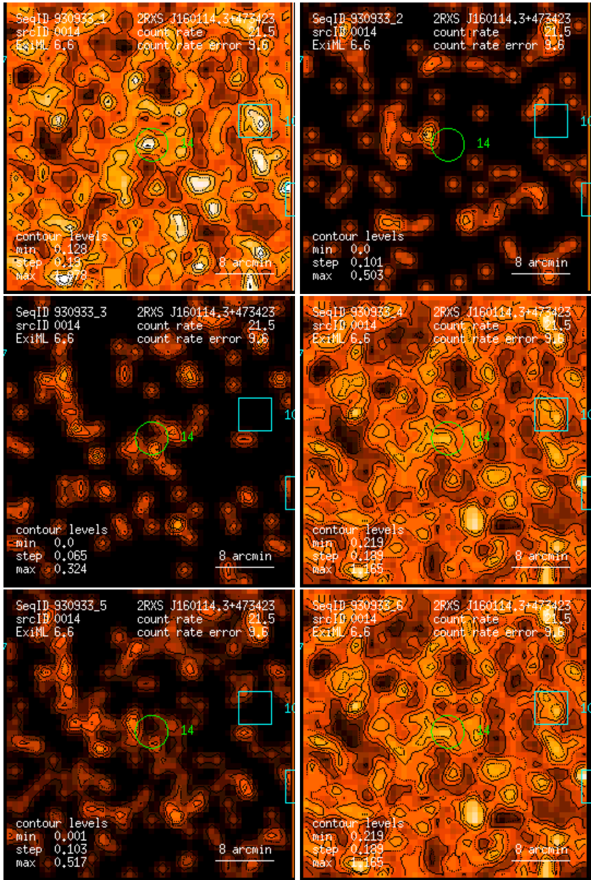
Figure 14: RASS 930933: detection 0014: band rate images, Gaussian filter: (1) PSPC channels 11 – 41, (2) 52 – 90, (3) 91 – 201, (4) 11 – 235, (5) 52 – 201, (6) 11 – 201. Broad band rates in counts/ks. Band rate contour levels in counts/ks/arcmin 2 .
