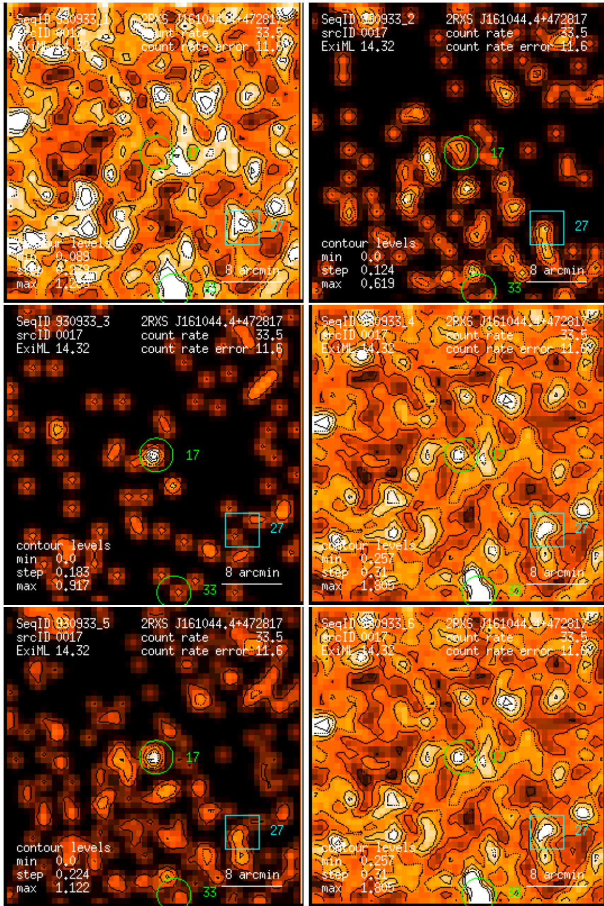
Figure 17: RASS 930933: detection 0017: band rate images, Gaussian filter: (1) PSPC channels 11 – 41, (2) 52 – 90, (3) 91 – 201, (4) 11 – 235, (5) 52 – 201, (6) 11 – 201. Broad band rates in counts/ks. Band rate contour levels in counts/ks/arcmin 2 .
