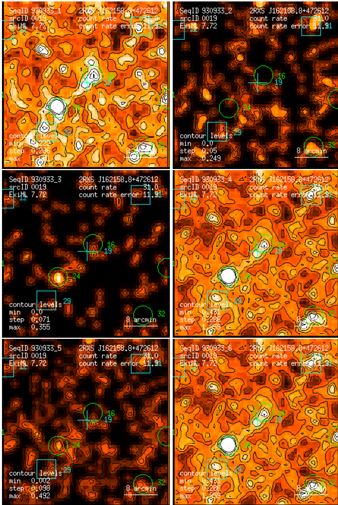
Figure 19: RASS 930933: detection 0019: band rate images, Gaussian filter: (1) PSPC channels 11 – 41, (2) 52 – 90, (3) 91 – 201, (4) 11 – 235, (5) 52 – 201, (6) 11 – 201. Broad band rates in counts/ks. Band rate contour levels in counts/ks/arcmin 2 .
