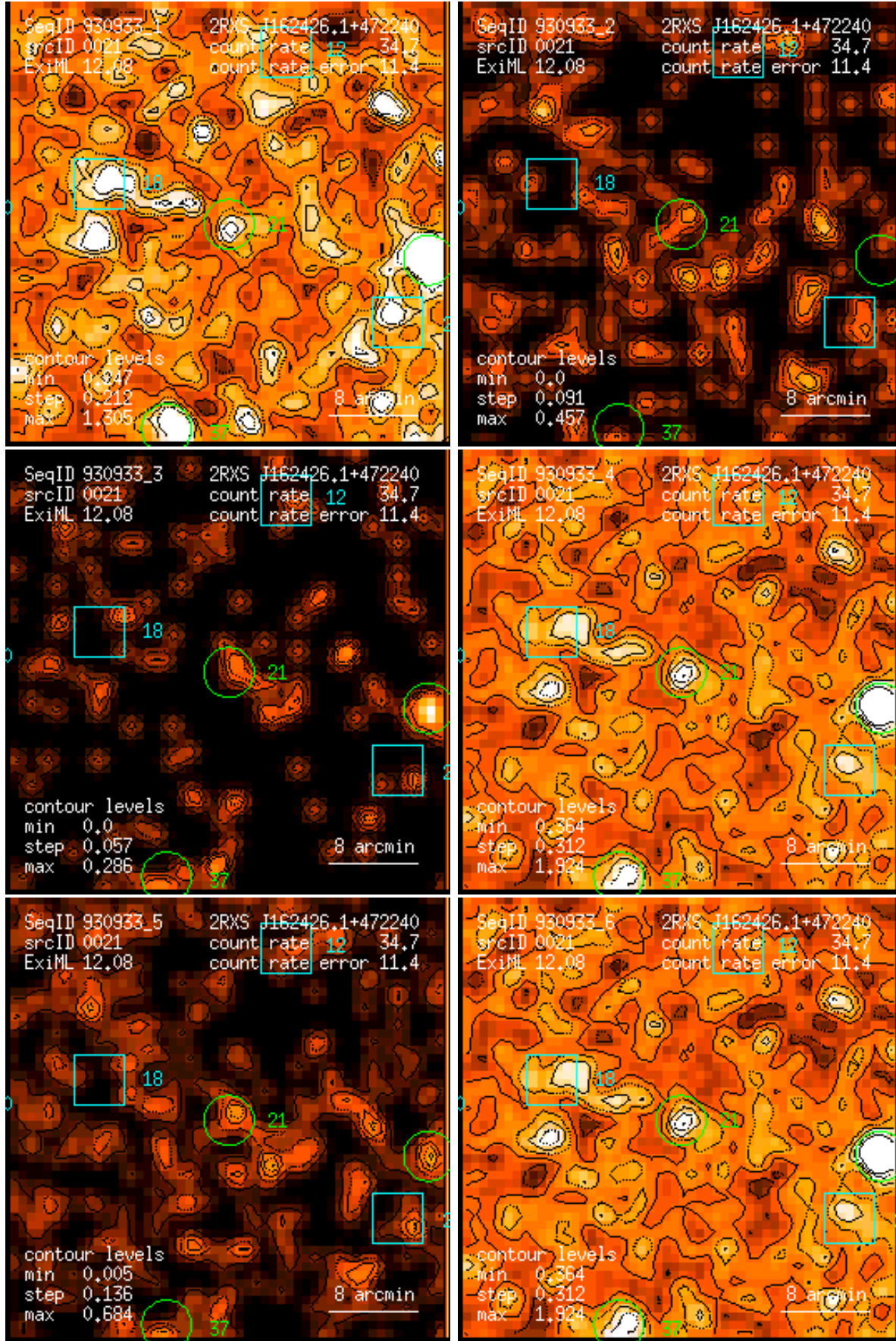
Figure 21: RASS 930933: detection 0021: band rate images, Gaussian filter: (1) PSPC channels 11 – 41, (2) 52 – 90, (3) 91 – 201, (4) 11 – 235, (5) 52 – 201, (6) 11 – 201. Broad band rates in counts/ks. Band rate contour levels in counts/ks/arcmin 2 .
