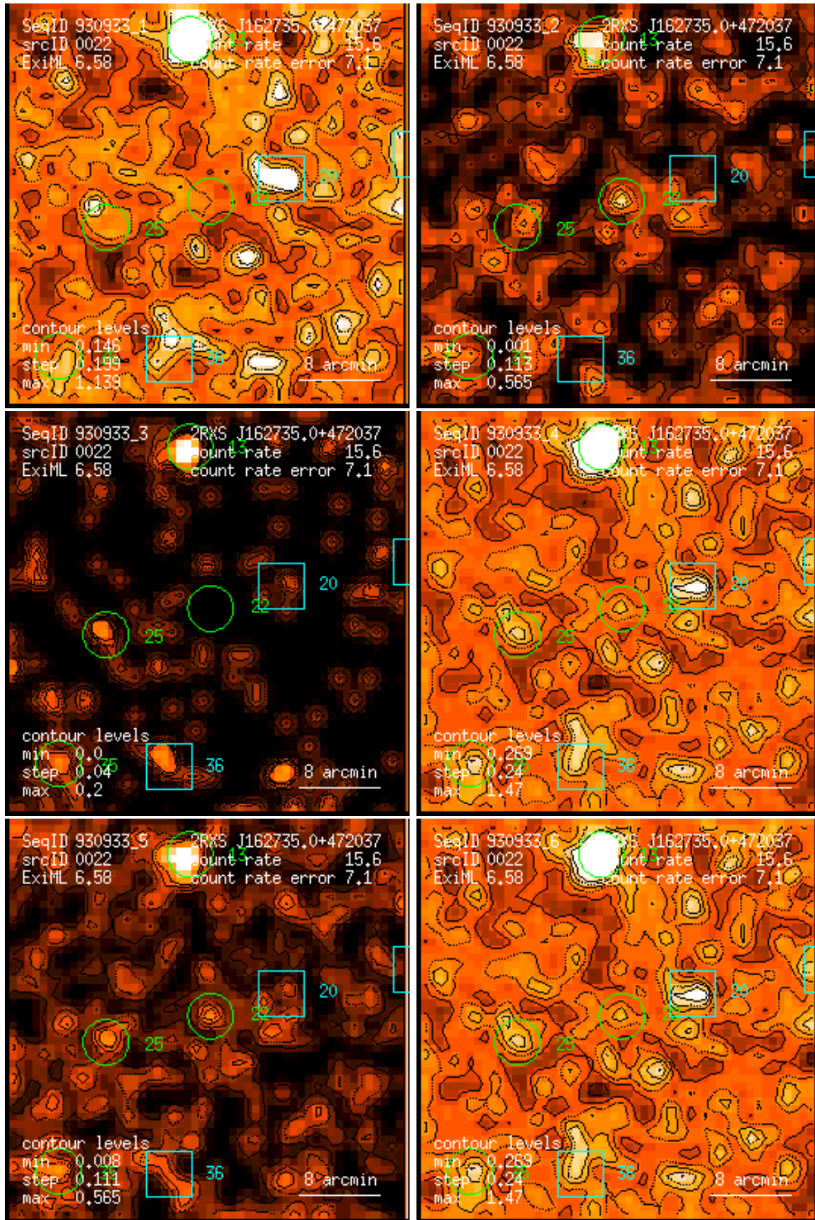
Figure 22: RASS 930933: detection 0022: band rate images, Gaussian filter: (1) PSPC channels 11 – 41, (2) 52 – 90, (3) 91 – 201, (4) 11 – 235, (5) 52 – 201, (6) 11 – 201. Broad band rates in counts/ks. Band rate contour levels in counts/ks/arcmin 2 .
