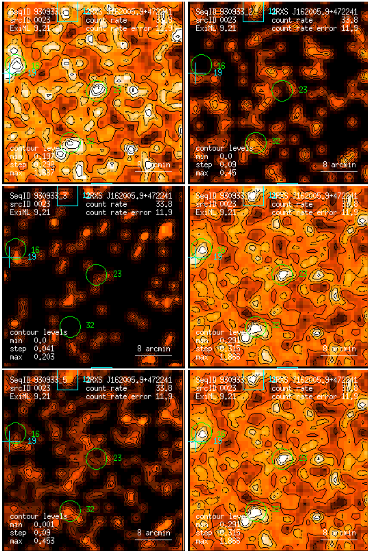
Figure 23: RASS 930933: detection 0023: band rate images, Gaussian filter: (1) PSPC channels 11 – 41, (2) 52 – 90, (3) 91 – 201, (4) 11 – 235, (5) 52 – 201, (6) 11 – 201. Broad band rates in counts/ks. Band rate contour levels in counts/ks/arcmin 2 .
