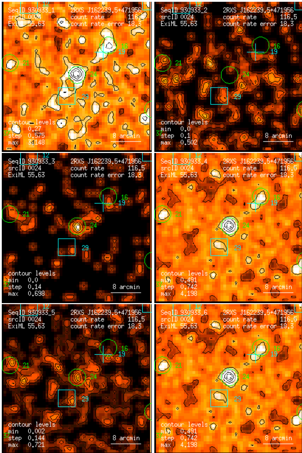
Figure 24: RASS 930933: detection 0024: band rate images, Gaussian filter: (1) PSPC channels 11 – 41, (2) 52 – 90, (3) 91 – 201, (4) 11 – 235, (5) 52 – 201, (6) 11 – 201. Broad band rates in counts/ks. Band rate contour levels in counts/ks/arcmin 2 .
