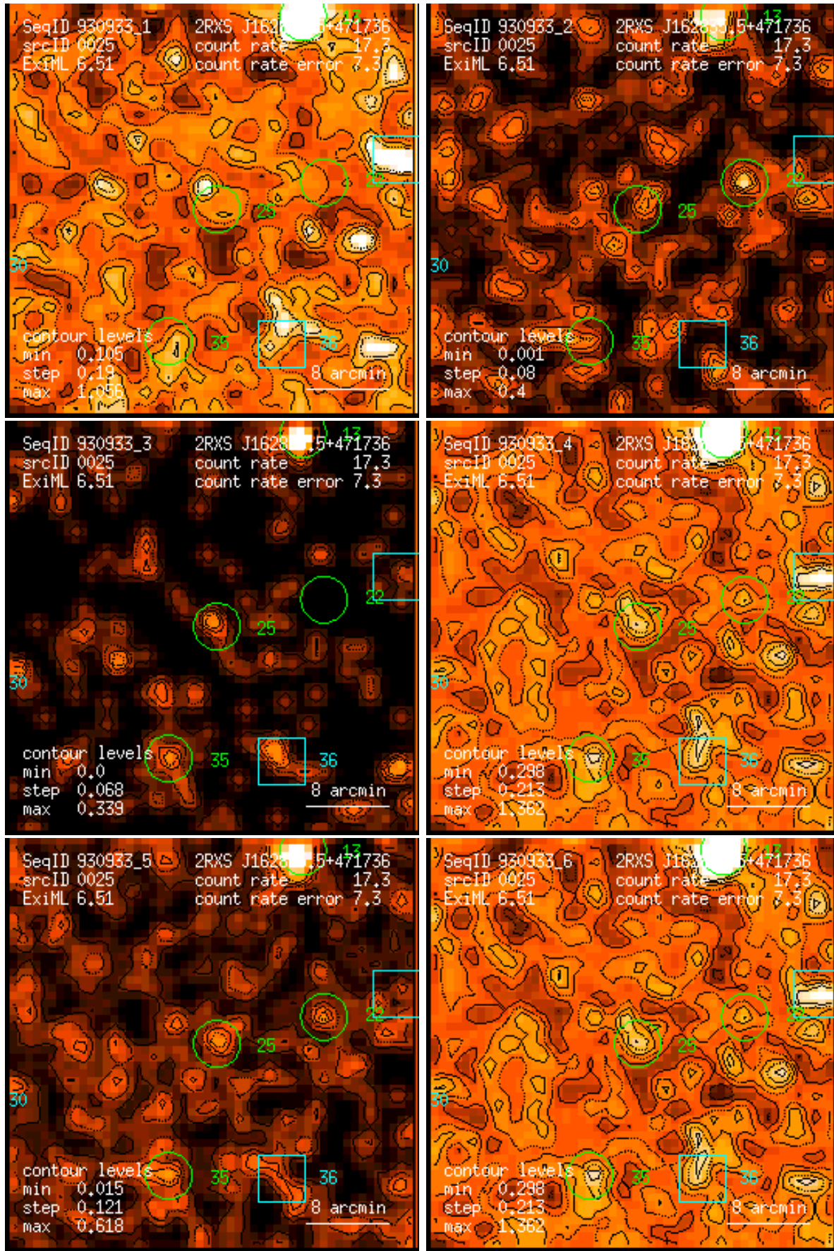
Figure 25: RASS 930933: detection 0025: band rate images, Gaussian filter: (1) PSPC channels 11 – 41, (2) 52 – 90, (3) 91 – 201, (4) 11 – 235, (5) 52 – 201, (6) 11 – 201. Broad band rates in counts/ks. Band rate contour levels in counts/ks/arcmin 2 .
