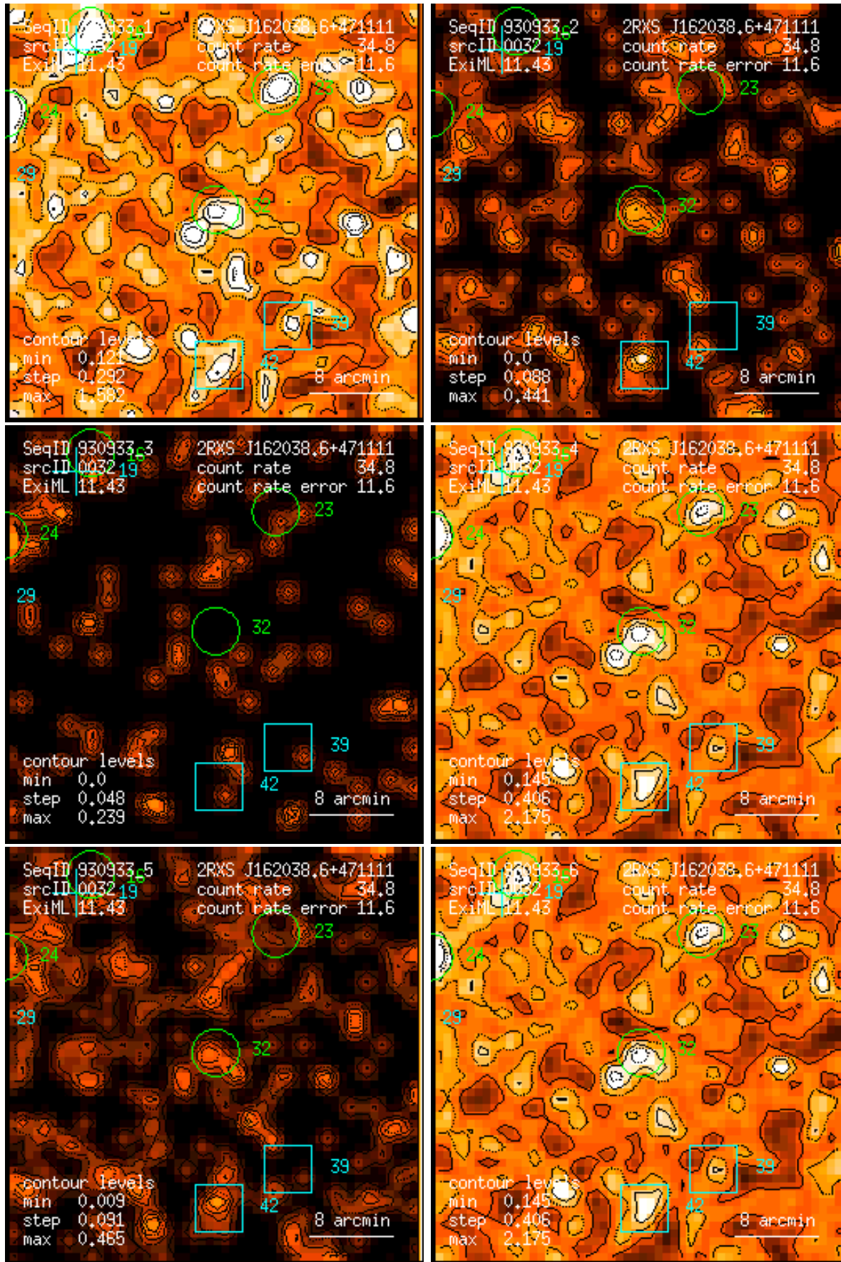
Figure 32: RASS 930933: detection 0032: band rate images, Gaussian filter: (1) PSPC channels 11 – 41, (2) 52 – 90, (3) 91 – 201, (4) 11 – 235, (5) 52 – 201, (6) 11 – 201. Broad band rates in counts/ks. Band rate contour levels in counts/ks/arcmin 2 .
