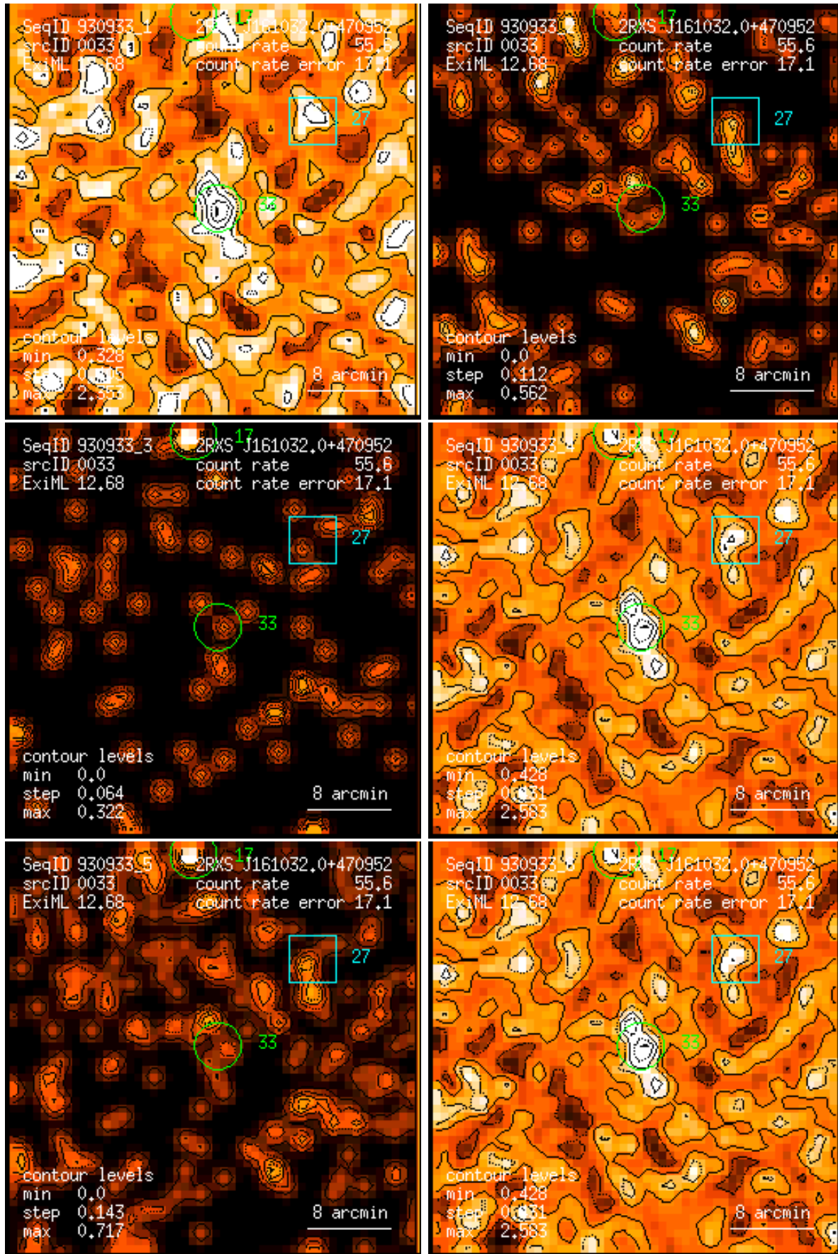
Figure 33: RASS 930933: detection 0033: band rate images, Gaussian filter: (1) PSPC channels 11 – 41, (2) 52 – 90, (3) 91 – 201, (4) 11 – 235, (5) 52 – 201, (6) 11 – 201. Broad band rates in counts/ks. Band rate contour levels in counts/ks/arcmin 2 .
