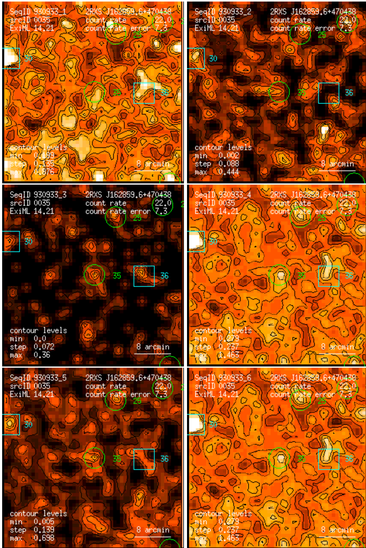
Figure 35: RASS 930933: detection 0035: band rate images, Gaussian filter: (1) PSPC channels 11 – 41, (2) 52 – 90, (3) 91 – 201, (4) 11 – 235, (5) 52 – 201, (6) 11 – 201. Broad band rates in counts/ks. Band rate contour levels in counts/ks/arcmin 2 .
