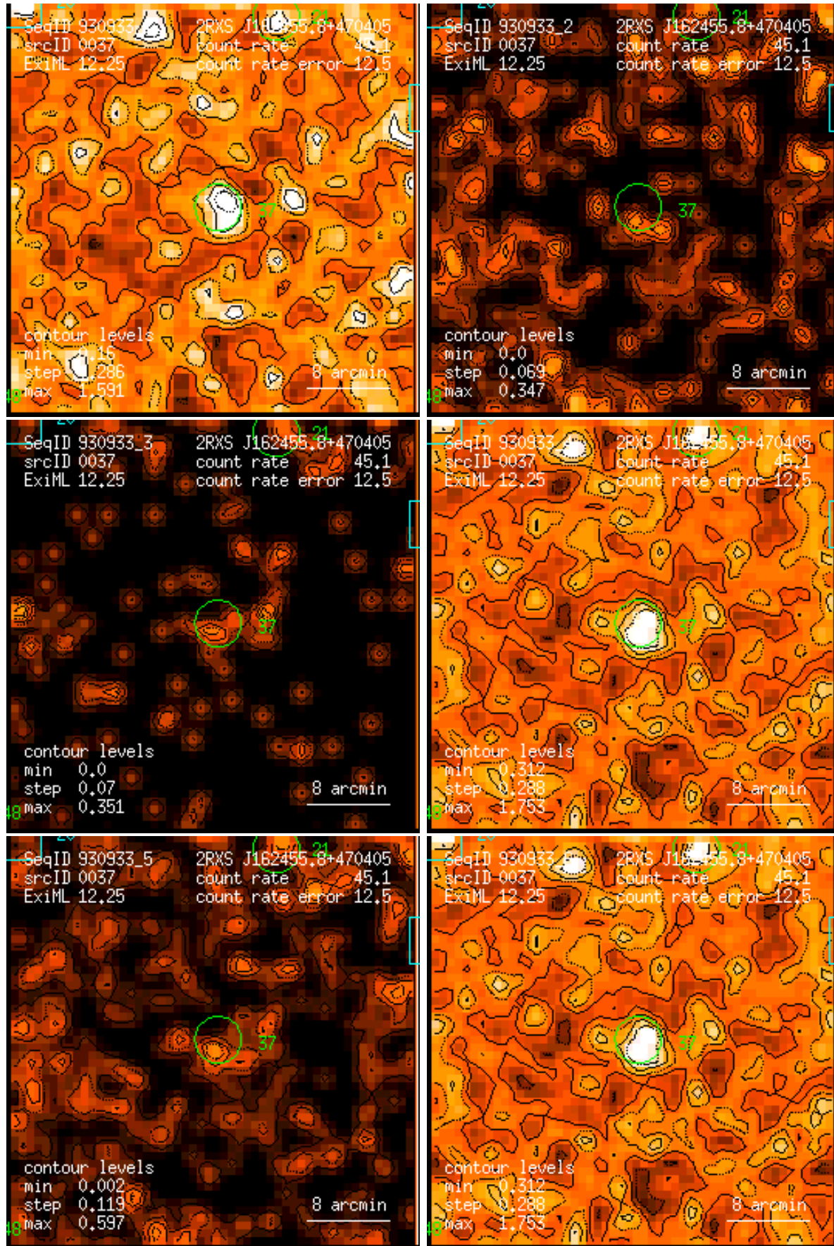
Figure 37: RASS 930933: detection 0037: band rate images, Gaussian filter: (1) PSPC channels 11 – 41, (2) 52 – 90, (3) 91 – 201, (4) 11 – 235, (5) 52 – 201, (6) 11 – 201. Broad band rates in counts/ks. Band rate contour levels in counts/ks/arcmin 2 .
