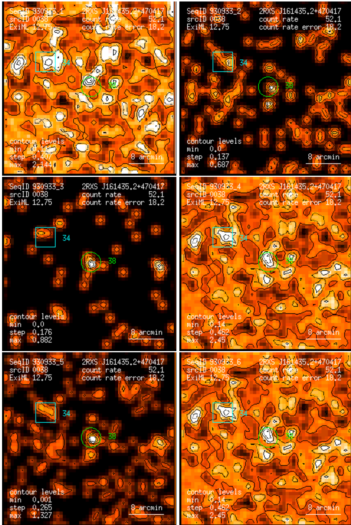
Figure 38: RASS 930933: detection 0038: band rate images, Gaussian filter: (1) PSPC channels 11 – 41, (2) 52 – 90, (3) 91 – 201, (4) 11 – 235, (5) 52 – 201, (6) 11 – 201. Broad band rates in counts/ks. Band rate contour levels in counts/ks/arcmin 2 .
