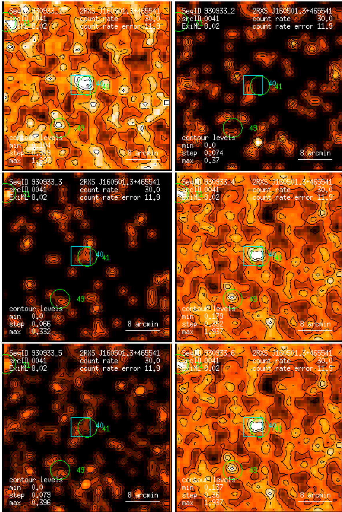
Figure 41: RASS 930933: detection 0041: band rate images, Gaussian filter: (1) PSPC channels 11 – 41, (2) 52 – 90, (3) 91 – 201, (4) 11 – 235, (5) 52 – 201, (6) 11 – 201. Broad band rates in counts/ks. Band rate contour levels in counts/ks/arcmin 2 .
