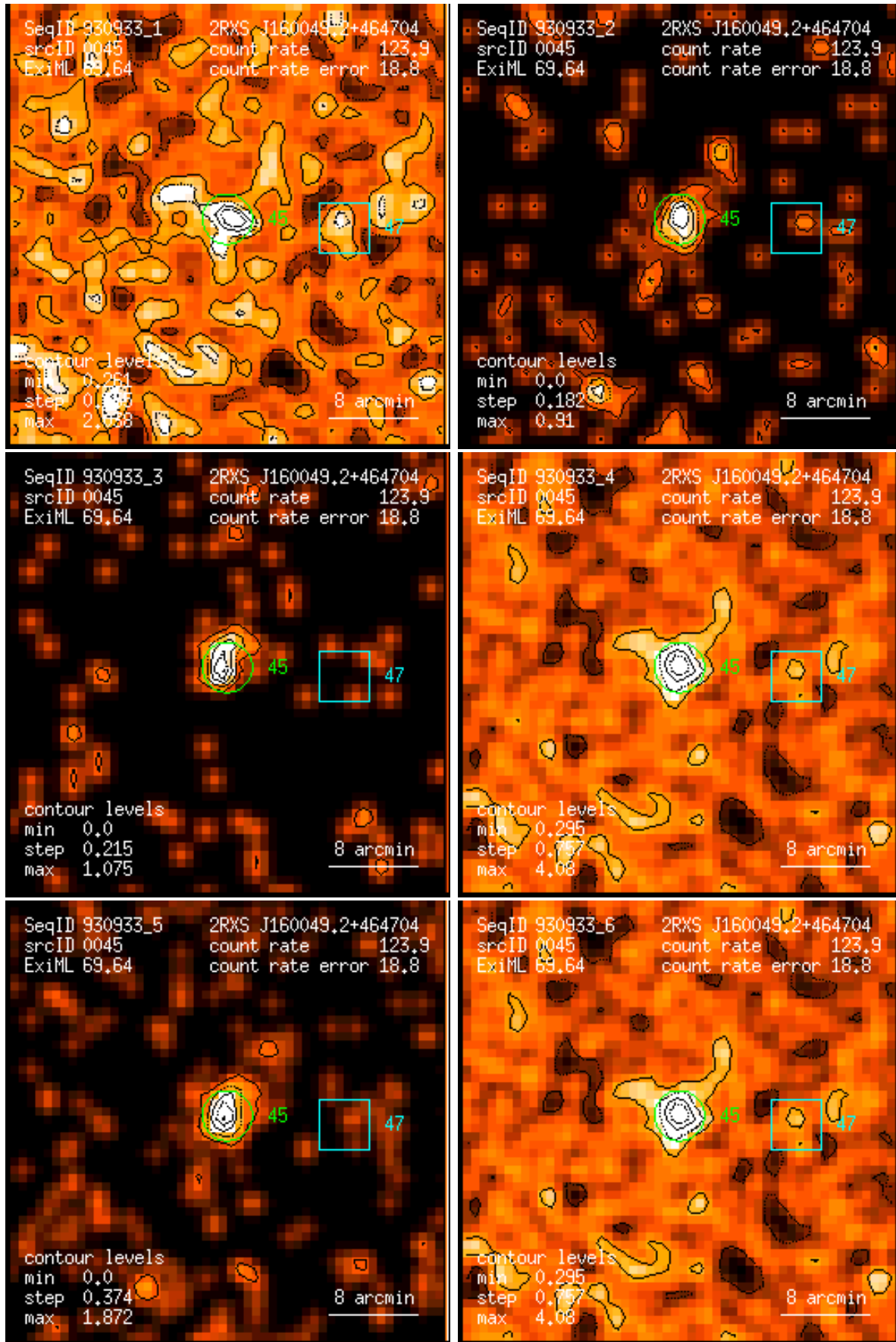
Figure 45: RASS 930933: detection 0045: band rate images, Gaussian filter: (1) PSPC channels 11 – 41, (2) 52 – 90, (3) 91 – 201, (4) 11 – 235, (5) 52 – 201, (6) 11 – 201. Broad band rates in counts/ks. Band rate contour levels in counts/ks/arcmin 2 .
