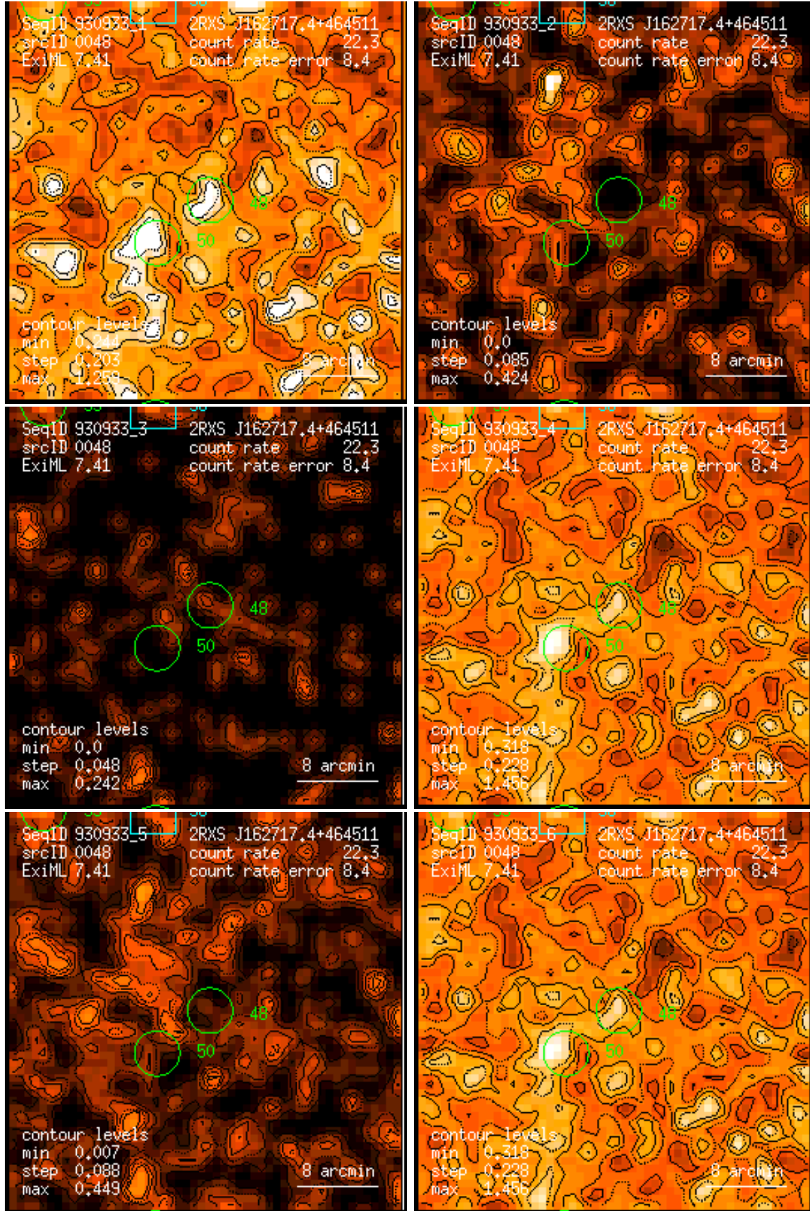
Figure 48: RASS 930933: detection 0048: band rate images, Gaussian filter: (1) PSPC channels 11 – 41, (2) 52 – 90, (3) 91 – 201, (4) 11 – 235, (5) 52 – 201, (6) 11 – 201. Broad band rates in counts/ks. Band rate contour levels in counts/ks/arcmin 2 .
