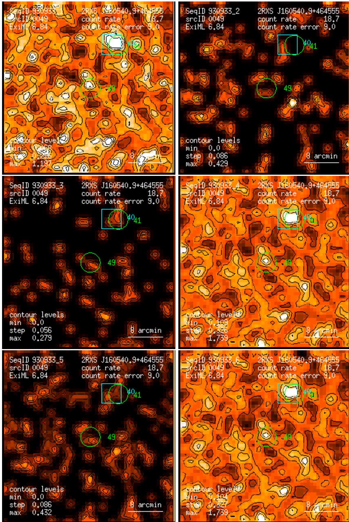
Figure 49: RASS 930933: detection 0049: band rate images, Gaussian filter: (1) PSPC channels 11 – 41, (2) 52 – 90, (3) 91 – 201, (4) 11 – 235, (5) 52 – 201, (6) 11 – 201. Broad band rates in counts/ks. Band rate contour levels in counts/ks/arcmin 2 .
