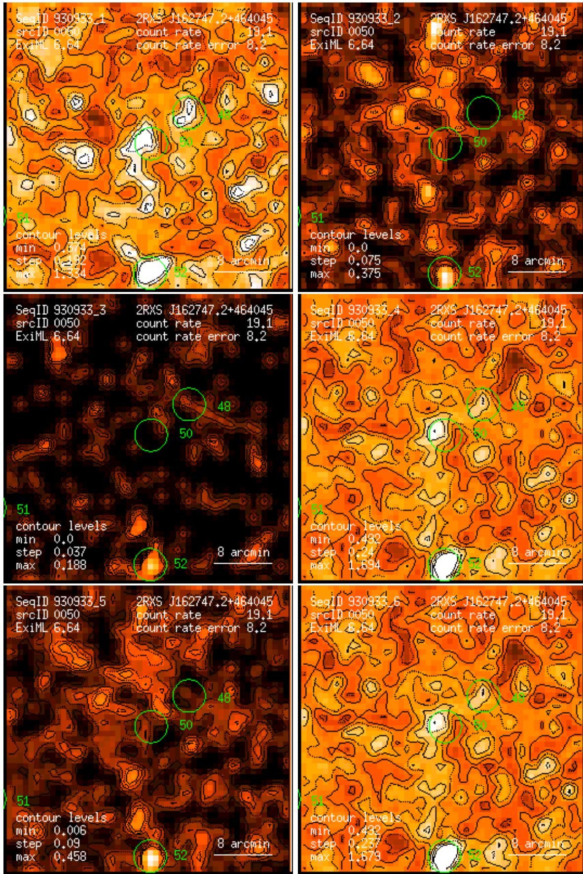
Figure 50: RASS 930933: detection 0050: band rate images, Gaussian filter: (1) PSPC channels 11 – 41, (2) 52 – 90, (3) 91 – 201, (4) 11 – 235, (5) 52 – 201, (6) 11 – 201. Broad band rates in counts/ks. Band rate contour levels in counts/ks/arcmin 2 .
