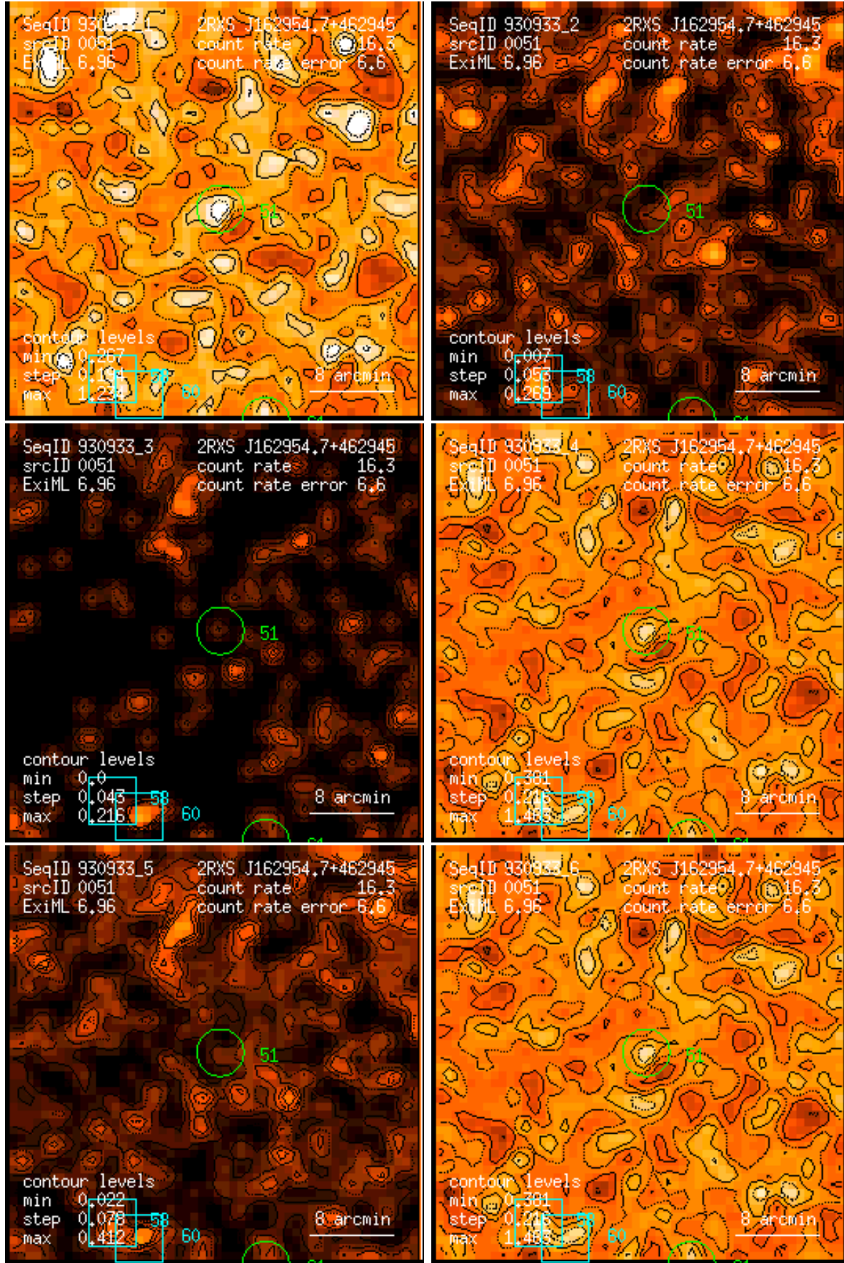
Figure 51: RASS 930933: detection 0051: band rate images, Gaussian filter: (1) PSPC channels 11 – 41, (2) 52 – 90, (3) 91 – 201, (4) 11 – 235, (5) 52 – 201, (6) 11 – 201. Broad band rates in counts/ks. Band rate contour levels in counts/ks/arcmin 2 .
