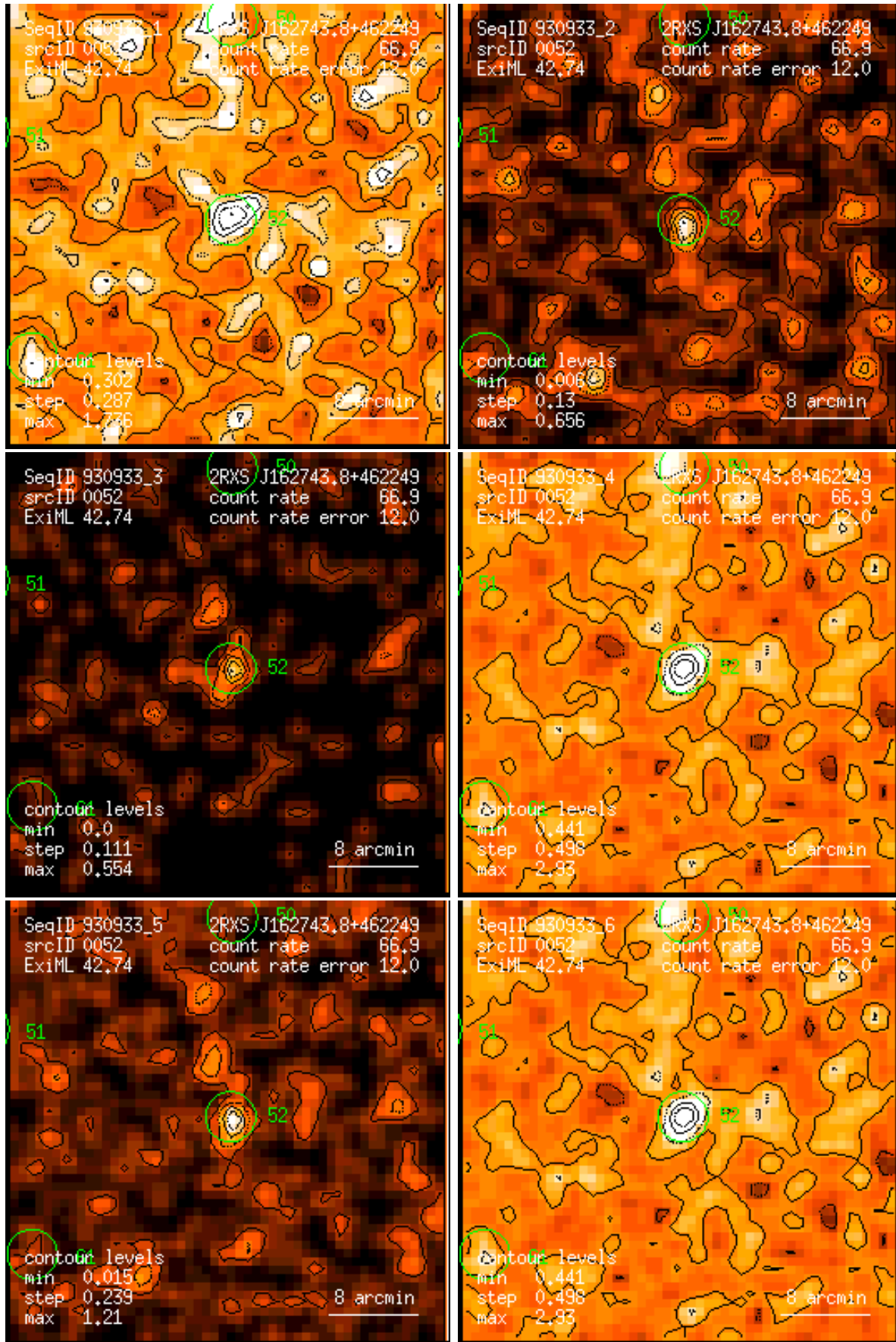
Figure 52: RASS 930933: detection 0052: band rate images, Gaussian filter: (1) PSPC channels 11 – 41, (2) 52 – 90, (3) 91 – 201, (4) 11 – 235, (5) 52 – 201, (6) 11 – 201. Broad band rates in counts/ks. Band rate contour levels in counts/ks/arcmin 2 .
