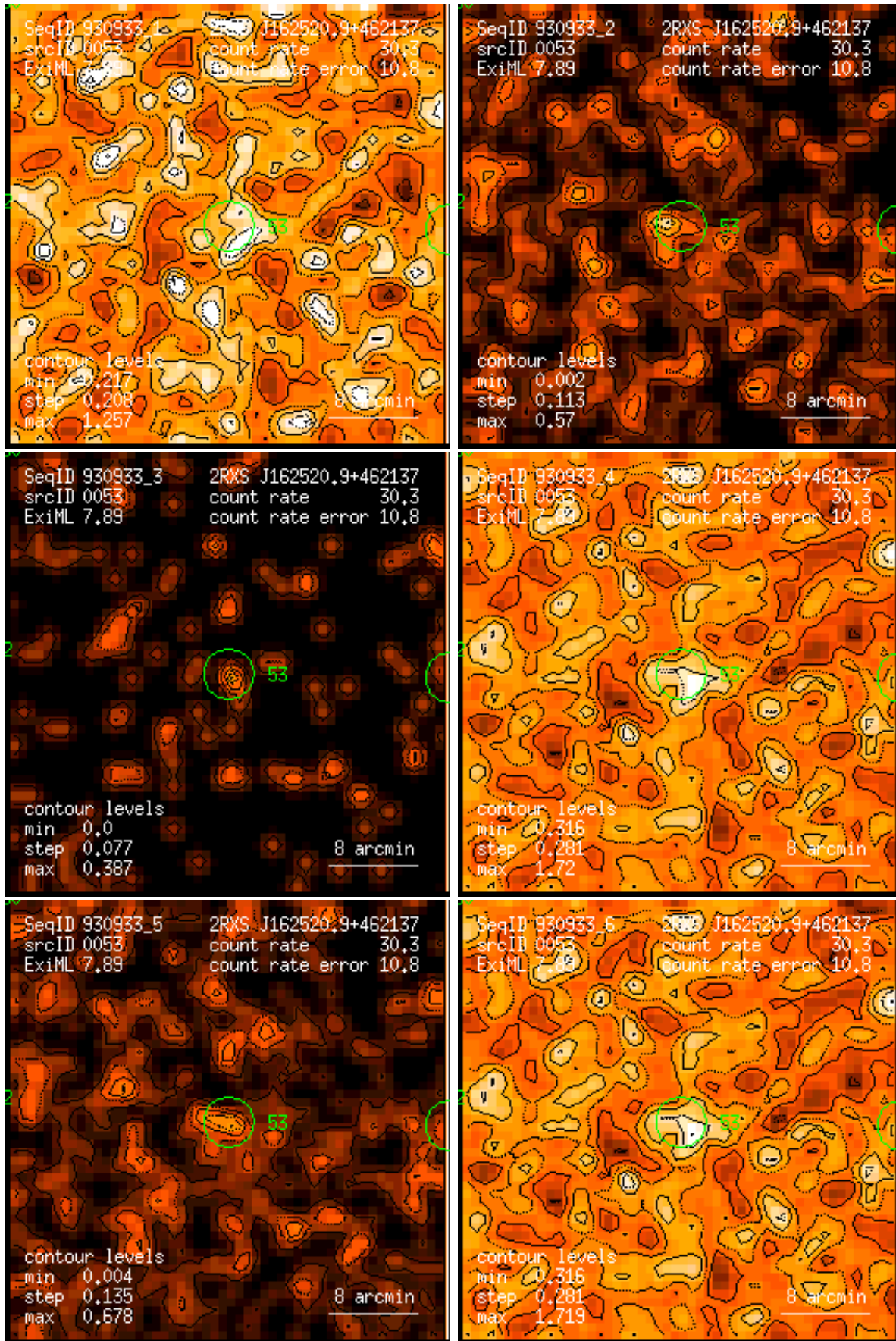
Figure 53: RASS 930933: detection 0053: band rate images, Gaussian filter: (1) PSPC channels 11 – 41, (2) 52 – 90, (3) 91 – 201, (4) 11 – 235, (5) 52 – 201, (6) 11 – 201. Broad band rates in counts/ks. Band rate contour levels in counts/ks/arcmin 2 .
