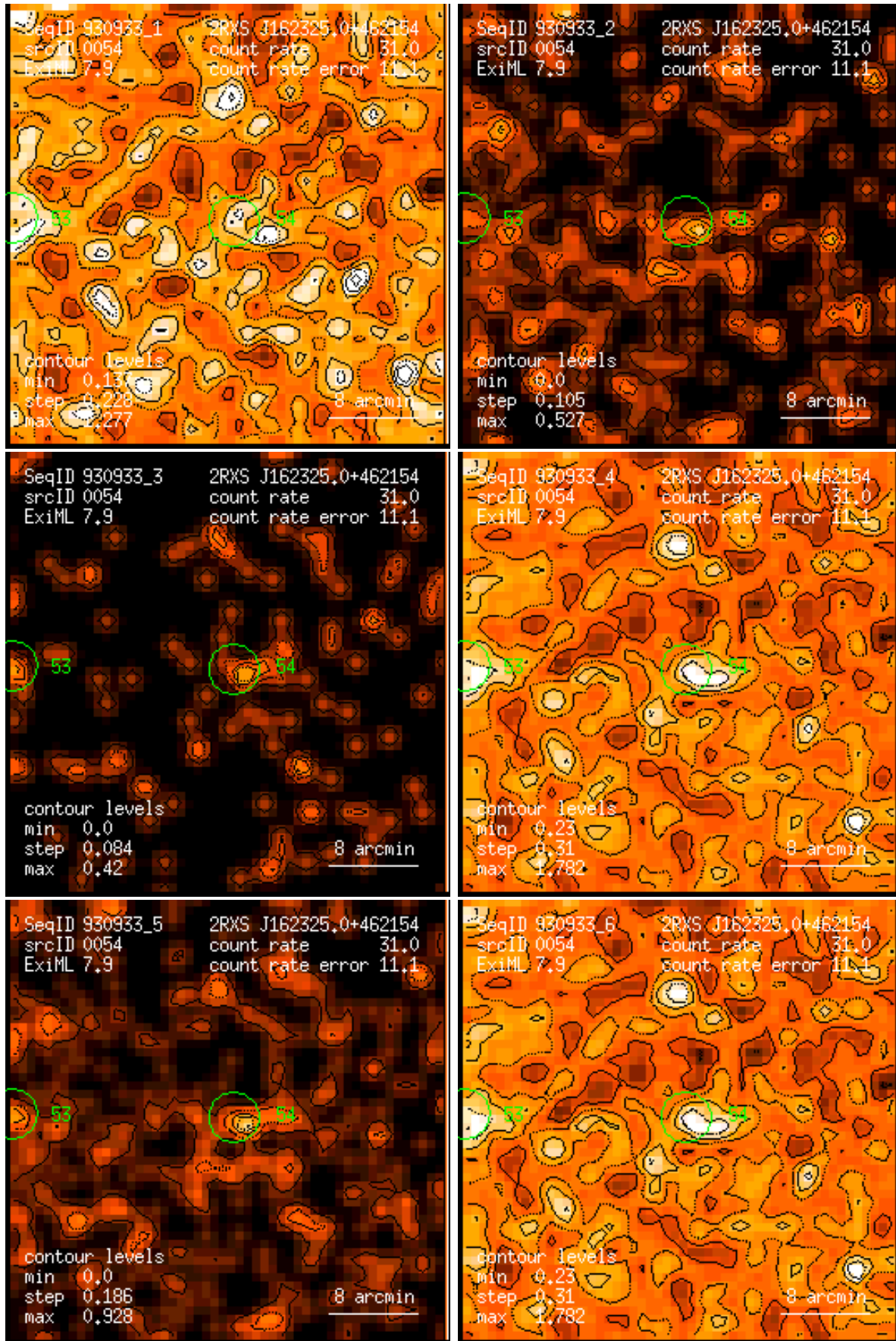
Figure 54: RASS 930933: detection 0054: band rate images, Gaussian filter: (1) PSPC channels 11 – 41, (2) 52 – 90, (3) 91 – 201, (4) 11 – 235, (5) 52 – 201, (6) 11 – 201. Broad band rates in counts/ks. Band rate contour levels in counts/ks/arcmin 2 .
