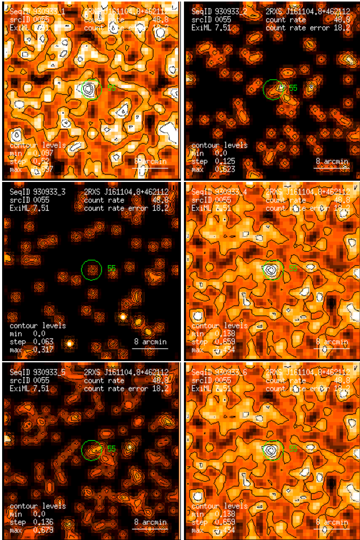
Figure 55: RASS 930933: detection 0055: band rate images, Gaussian filter: (1) PSPC channels 11 – 41, (2) 52 – 90, (3) 91 – 201, (4) 11 – 235, (5) 52 – 201, (6) 11 – 201. Broad band rates in counts/ks. Band rate contour levels in counts/ks/arcmin 2 .
