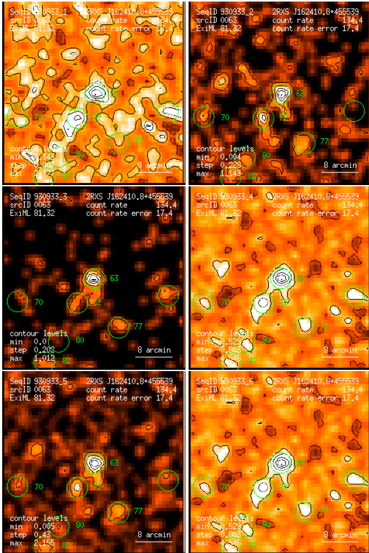
Figure 63: RASS 930933: detection 0063: band rate images, Gaussian filter: (1) PSPC channels 11 – 41, (2) 52 – 90, (3) 91 – 201, (4) 11 – 235, (5) 52 – 201, (6) 11 – 201. Broad band rates in counts/ks. Band rate contour levels in counts/ks/arcmin 2 .
