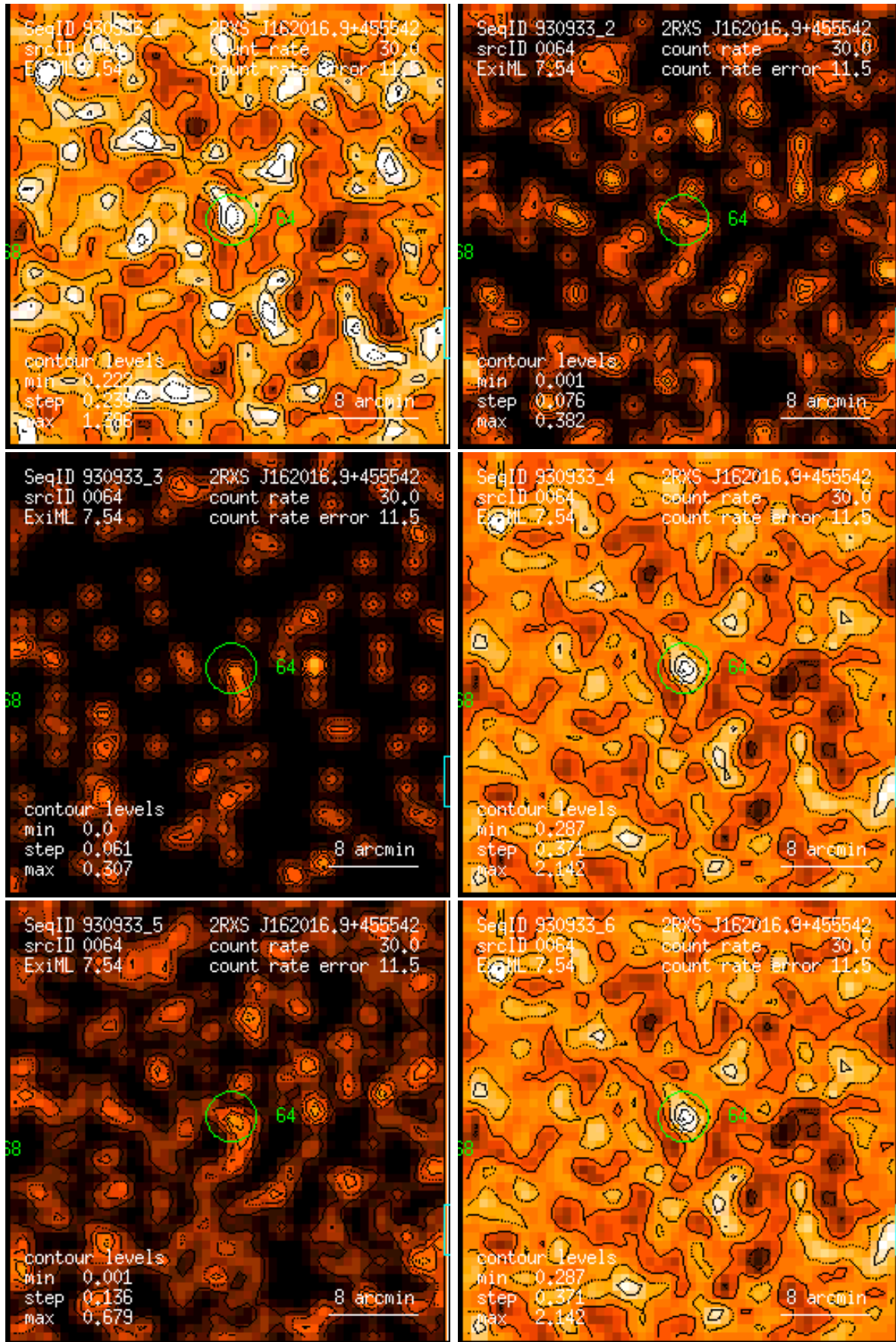
Figure 64: RASS 930933: detection 0064: band rate images, Gaussian filter: (1) PSPC channels 11 – 41, (2) 52 – 90, (3) 91 – 201, (4) 11 – 235, (5) 52 – 201, (6) 11 – 201. Broad band rates in counts/ks. Band rate contour levels in counts/ks/arcmin 2 .
