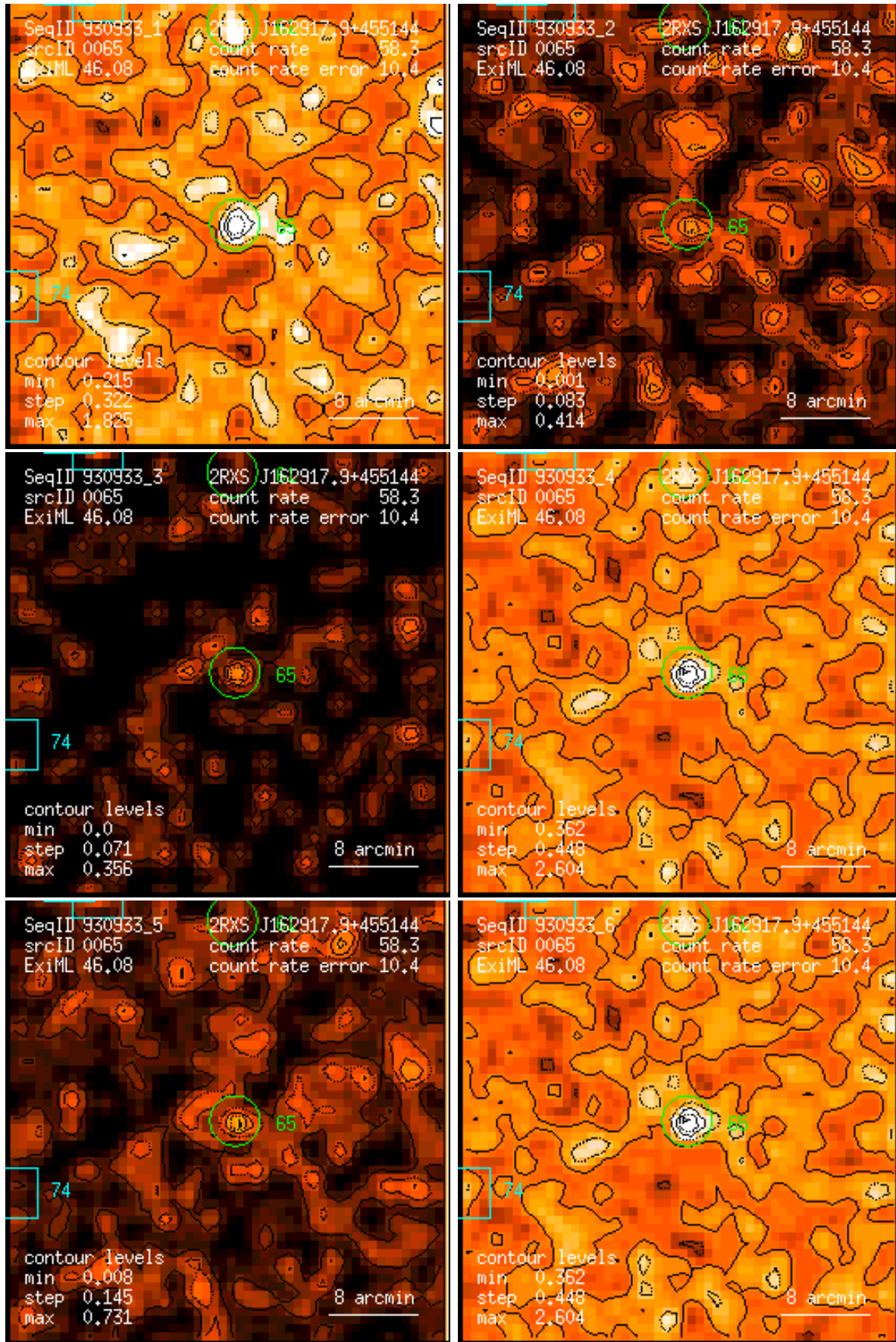
Figure 65: RASS 930933: detection 0065: band rate images, Gaussian filter: (1) PSPC channels 11 – 41, (2) 52 – 90, (3) 91 – 201, (4) 11 – 235, (5) 52 – 201, (6) 11 – 201. Broad band rates in counts/ks. Band rate contour levels in counts/ks/arcmin 2 .
