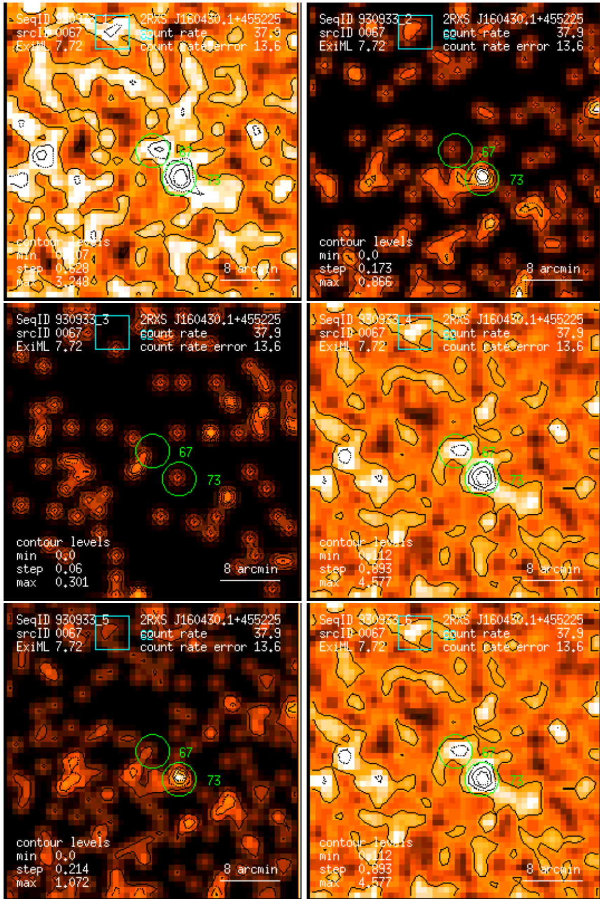
Figure 67: RASS 930933: detection 0067: band rate images, Gaussian filter: (1) PSPC channels 11 – 41, (2) 52 – 90, (3) 91 – 201, (4) 11 – 235, (5) 52 – 201, (6) 11 – 201. Broad band rates in counts/ks. Band rate contour levels in counts/ks/arcmin 2 .
