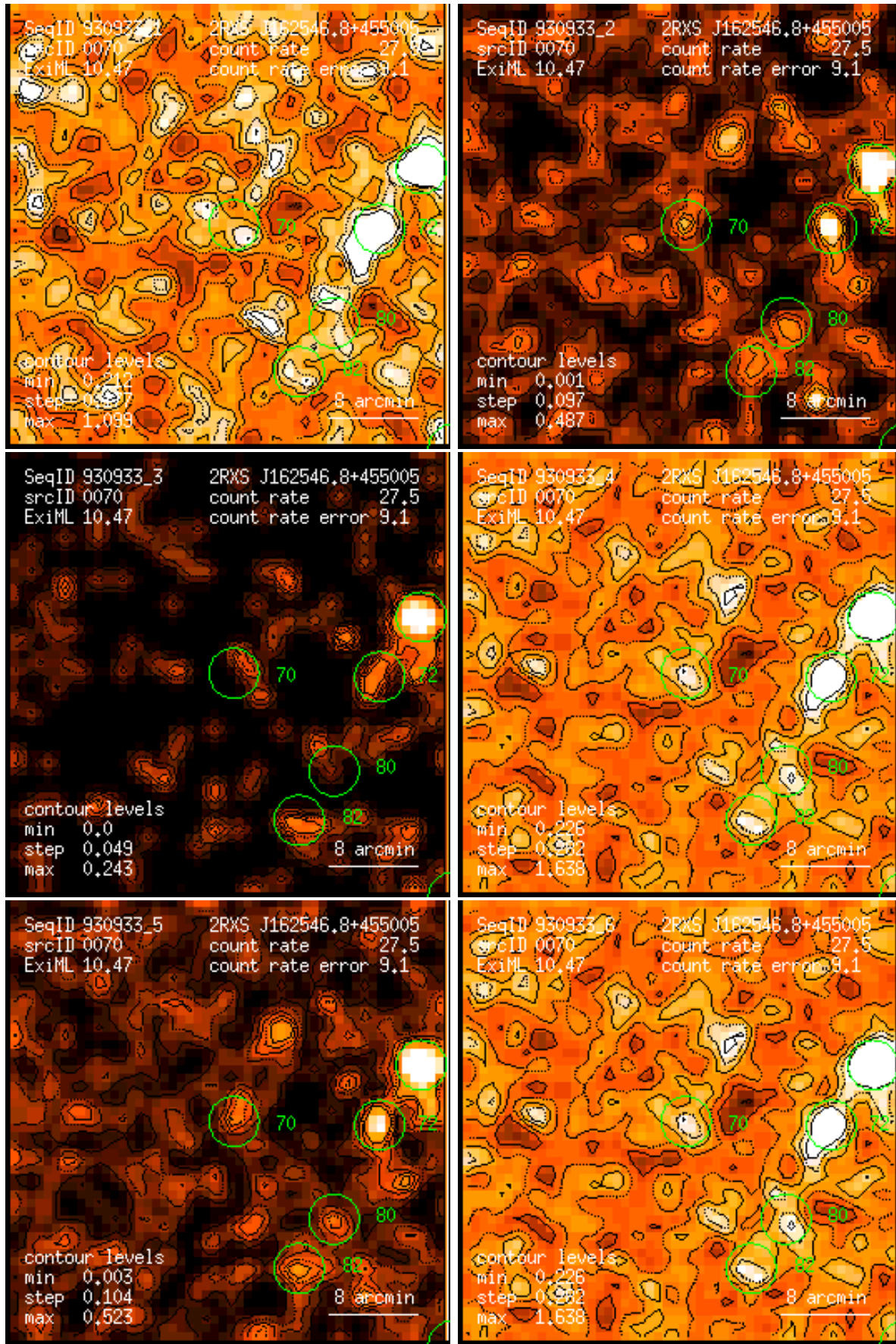
Figure 70: RASS 930933: detection 0070: band rate images, Gaussian filter: (1) PSPC channels 11 – 41, (2) 52 – 90, (3) 91 – 201, (4) 11 – 235, (5) 52 – 201, (6) 11 – 201. Broad band rates in counts/ks. Band rate contour levels in counts/ks/arcmin 2 .
