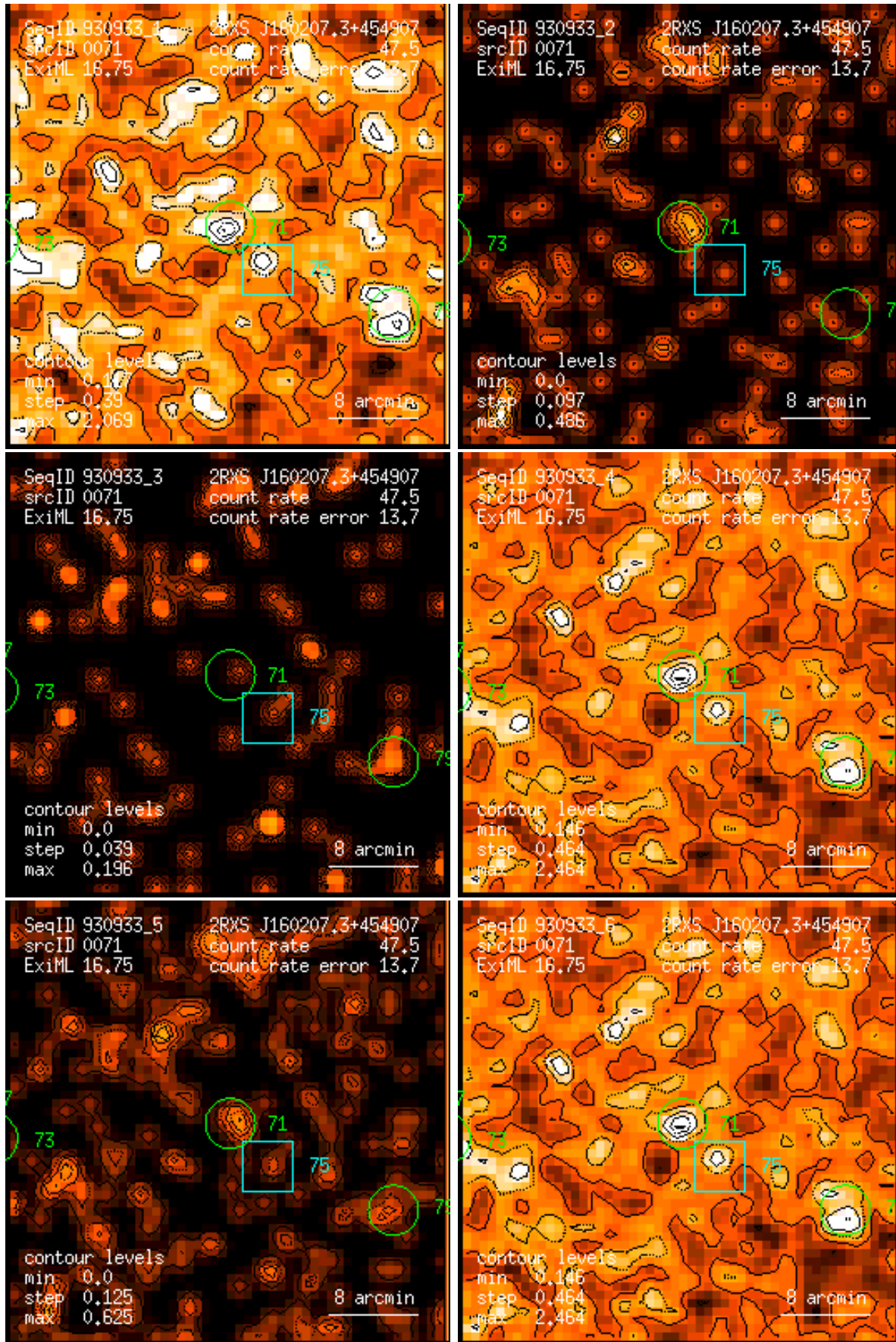
Figure 71: RASS 930933: detection 0071: band rate images, Gaussian filter: (1) PSPC channels 11 – 41, (2) 52 – 90, (3) 91 – 201, (4) 11 – 235, (5) 52 – 201, (6) 11 – 201. Broad band rates in counts/ks. Band rate contour levels in counts/ks/arcmin 2 .
